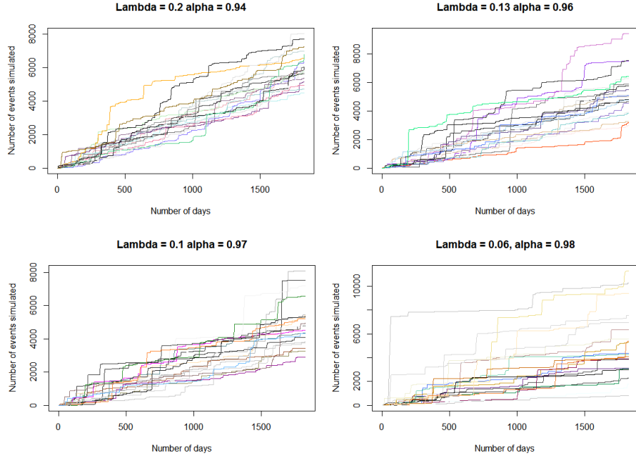
Figure 8: Simulation of 20 trajectories over five years for four set of parameters
