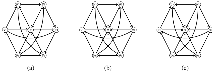
Figure 3: (a): the digraph D_7 ; (b): the digraph D_7^l obtained from D_7 inverting the set \{y, y_2, y_4, y_6\} ; (c): the acyclic digraph D_7^l obtained from D_7^l by inverting the set \{y_2, y_3, y_5, y_6\} .
