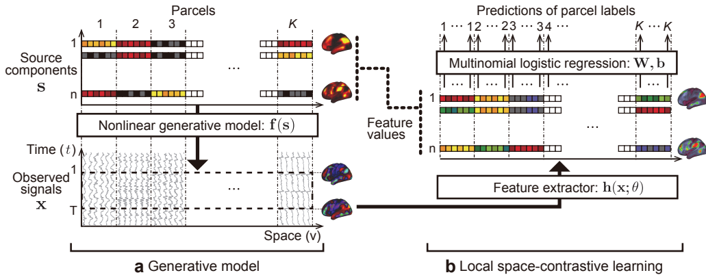
Figure 1: The concept of local space-contrastive learning (LSCL). (a) The generative model is basically a nonlinear version of sICA. The source components are spatial patterns which are spatially (conditionally) mutually independent. The observed time series are given by a nonlinear transformation of the components for each location. Different from ordinary sICA, the components have spatial-parcel-wise stationarity, i.e. different statistics in different parcels, and spatial-parcel-wise independence, which does not necessary mean marginal independence generally assumed in sICA. In addition, LSCL assumes that the components generating the time series can be different for each short temporal window (dotted rectangle on the observed signals), which is in contrast to ordinary sICA, which assumes that the whole time series are generated from the common components. (b) In LSCL, we attempt to find the original components by training a feature extractor to be sensitive to the spatial nonstationarity of the data by using a multinomial logistic regression. The feature extractor is given a short fragment of time series randomly picked from the whole time series at a location as an input, and the logistic regression attempts to predict the parcel label ( 1, \dots, K ) corresponding to it from the output of the feature extractor (feature values). This framework makes the feature extractor learn component-specific local nonlinear temporal structures, referred to as temporal primitives . See Inline Supplementary Fig. 5 for the detailed procedures to obtain the feature values, which are described in Section 2.5 .
