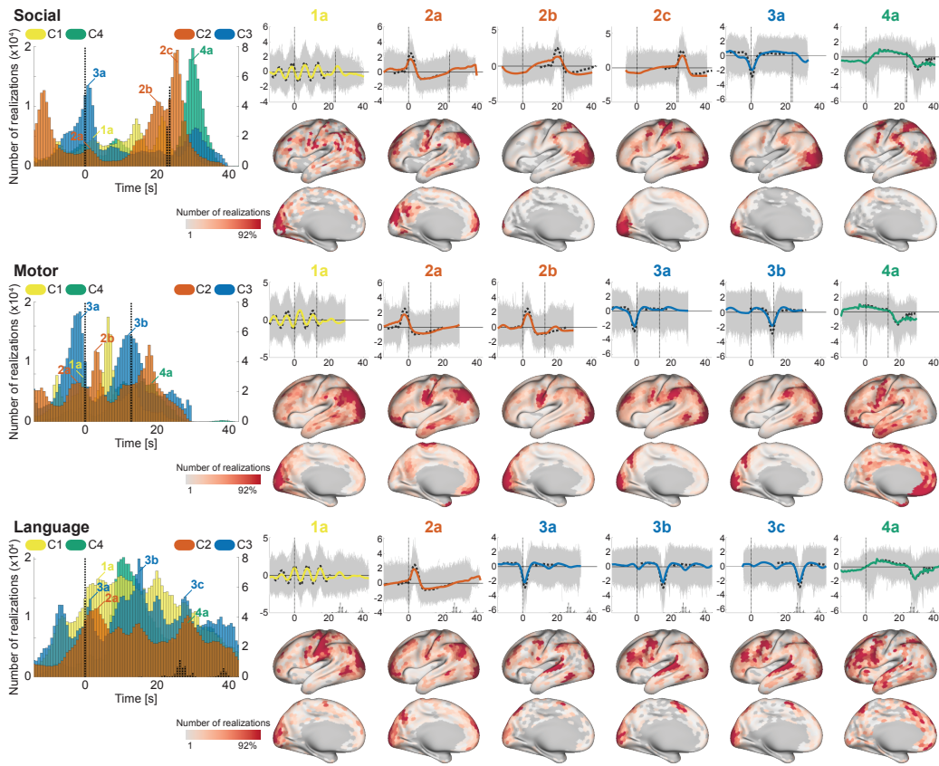
Figure 8: The timings and spatial locations of the realizations during the task conditions (Social, Motor, and Language). See Fig. 7 for the details.
