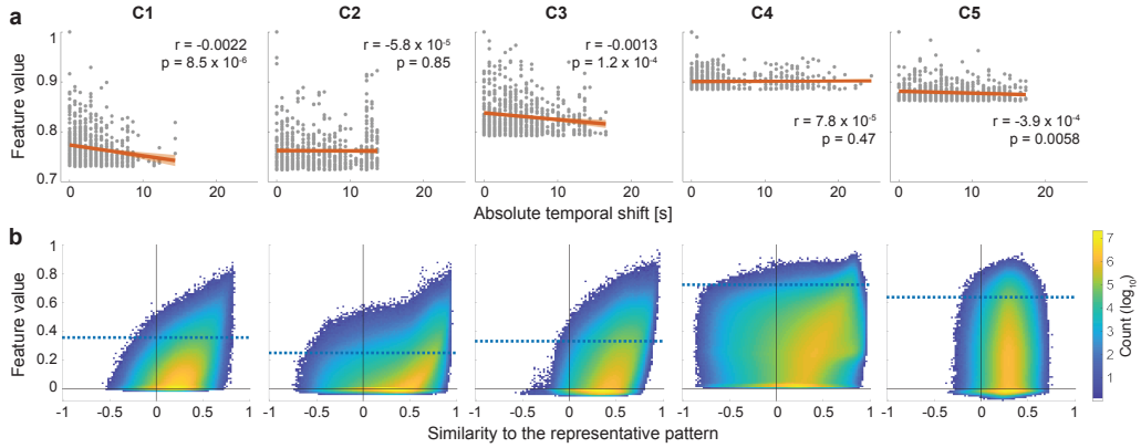
Figure 4: Invariance of the feature extractor against temporal modulations of the temporal primitives. (a) The robustness of the feature extractor to the temporal shifts of the realizations. Each panel shows the relationship between the feature values and the (absolute) temporal shifts that were applied to their inputs for alignment to reference signal in Fig. 2a. Each point corresponds to one of the top time series shown in Fig. 2a ( n = 695 ). The feature values were normalized to have maximum value of 1 for each component. The red lines are the estimated least-square fits, and colored bands indicate 95% confidence bounds. Although the slopes are significant in some of the components, they are quite small, which illustrates the shift-invariance of the feature extractor. (b) Two-dimensional histogram showing the relationship between feature values and the similarities of their inputs to the representation patterns (Fig. 2a). To evaluate only the modulations different from the temporal shifts shown in a , the similarities (Pearson correlation) were measured after compensating their temporal shifts relative to the representative patterns (see Section 2.8 for the temporal-shift alignment). Blue horizontal lines are the chance levels same with those shown in Fig. 3a. Note that the colorbar is log-scale.
