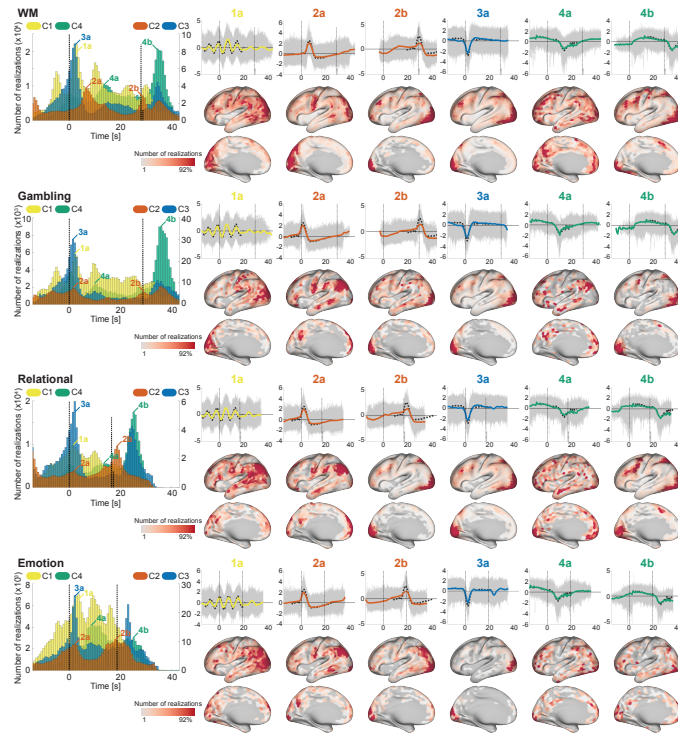
Figure 7: The timings and spatial locations of the realizations during the task conditions (WM, Gambling, Relational, and Emotion; see the remaining task conditions in Fig. 8). We discarded C5 here because of the lack of temporal preferences. (Left) Histogram of the timings of the realizations of the components (see Section 2.12 for more details). One temporal bin corresponds to one volume. Although there are some sub-conditions for each task, we mixed all of their realizations as the same task (Motor-CUE condition was excluded). The vertical line at 0 s indicates the onset of the task block, and the other vertical lines show the end of the task blocks. The length of the vertical lines indicates the number (ratio) of blocks ended at the timing. Note that the width of the receptive field of the feature extractor (about 32 s) is longer than the length of task blocks. (Right-upper) Temporal patterns of the realizations corresponding to some peaks on the histograms. Grey thin lines show the realizations corresponding to the timing, and the colored thick line is their sample average. Black dotted line shows the representative pattern obtained in Fig. 2a and used as a reference for estimating the timings. (Right-lower) Spatial histogram of the realizations on the specific timing given in the upper part.
