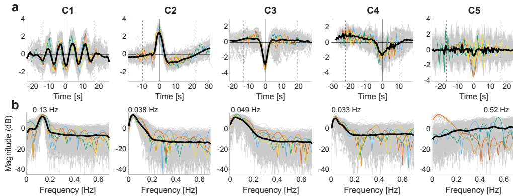
Figure 2: (a) Visualization of the representative temporal patterns (the most important temporal characteristics) of temporal primitives , which are component-specific spatio-temporally-local nonlinear temporal structures learned by the nonlinear feature extractor (CNN). They were represented by taking an average of time fragments whose (unmixed) feature values were very large at each component dimension. Gray thin lines are the individual input time series which produced the top-0.0001% highest component activities in the whole dataset. The colored thin lines indicate the samples with the very highest activations (1st–5th: red, orange, yellow, green, and blue). Considering the well-known property of shift-invariance of CNNs (see Fig. 4a for further evaluation), all samples were temporally shifted so as to maximize their cross correlations to the reference signal, i.e. the one with the highest activity (red sample). The black thick line shows their sample average after the temporal shifting. Two dotted vertical lines indicate the edges of a temporal window whose width is the same as the width of the receptive field of the feature extractor ( \sim 32 s); the (absolute) peak point inside the window was selected as the reference point (0 s). We can see that the average temporal patterns inside the windows show clear differences across components, and are hereafter used as the representative temporal patterns of the temporal primitives. (b) The representative frequency spectra of the temporal primitives. The spectrum was estimated for each of shift-adjusted inputs corresponding to those in a (see Section 2.9 for the shift-adjustment). As with a , the gray thin lines are the individual plots, the colored thin lines indicate the samples with the very highest activations, and the black thick line shows their average. The peak frequency of the average spectrum was displayed on the line.
