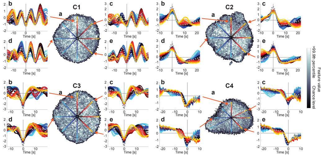
Figure 5: Visualization of the modulations of the temporal primitives. (a) two-dimensional t-SNE embedding of the realizations (see Section 2.9 for t-SNE analysis details). Each point corresponds to one of the realizations. The grayscale color indicates the feature value. Their chance levels (the lower bounds of the realizations) are the same as Fig. 3. (b–e) Each panel illustrates the temporal patterns of some local realizations, which were shown by gradually changing the location on a line on the embedded space. The colored cross on the t-SNE space indicates the sampling location, and the temporal pattern plotted with the same color in the corresponding panel shows the temporal pattern given by a local average of the 100 closest points around the location. The gray dotted line is the representative pattern obtained in Fig. 2a, which were used as a reference for compensating the temporal shifts of the realizations. Those differences of the temporal patterns in the embedded space illustrate the modulations of the realizations.
