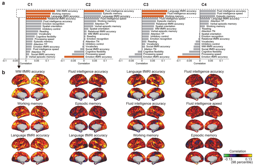
Figure 9: The relationship of the temporal primitives to the behavioral traits of the subjects. (a) Spearman correlation coefficient between subject-average component activities and 19 behavioral traits related to intelligence and response-accuracies during tfMRI. Red bars indicate significant relationship ( p < 0.05 ; 100,000 times permutation test, with FDR correction for multiple comparisons). (b) The spatial distribution of the relationship between subject-parcel-average component activities and some traits corresponding to the top-3 highest correlation in a for each component (column).
