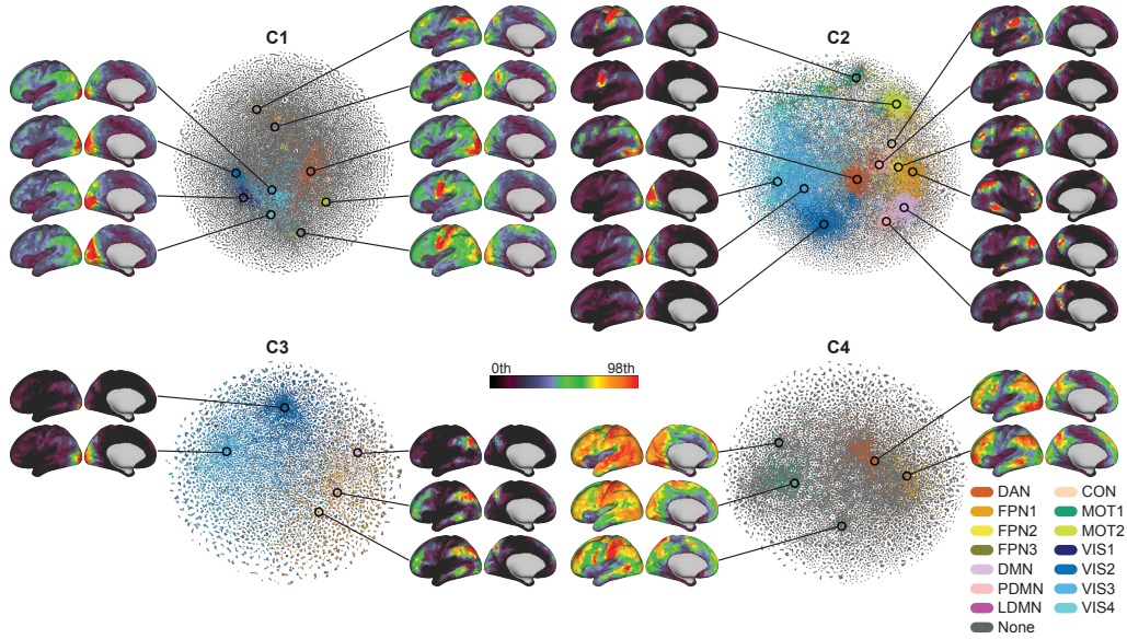
Figure 6: The spontaneous spatial co-occurrence patterns of the temporal primitives. Scatter plots show two-dimensional t-SNE embeddings of the spatial co-occurrence patterns of the temporal primitives during the resting-states (see Section 2.11 for t-SNE analysis details). The color indicates the most similar RSN obtained by conventional linear sICA (see Inline Supplementary Fig. 3); DAN (dorsal attention network), FPN (fronto-parietal network), DMN (default mode network), PDMN (posterior DMN), LDMN (lateral DMN), CON (cingulo-opercular network), MOT (motor and somatosensory network), and VIS (visual network). The similarities were measured by Pearson correlation, and thresholded by 0.35; the gray points have similarities to the RSNs less than 0.35. The spatial patterns show some examples of the co-occurrence patterns on the embedded space, obtained by taking local average of 500 data points on some locations. Only left hemispheres are shown, except for the FPN of C2 because it showed right dominant pattern.
