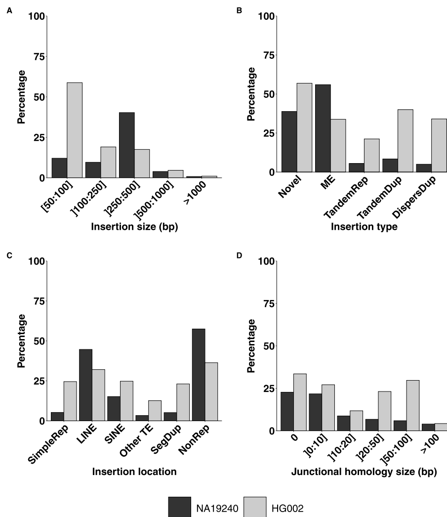
Fig. 4 Proportions of SR-based insertion discoveries according to insertion features. Proportions of insertions that were called using short read technology data according to a insertion size, b insertion type, c insertion location and d homology size at the breakpoint, in the NA19240 and HG002 callsets. These callsets were provided by two different studies using different discovery tools and methodologies
