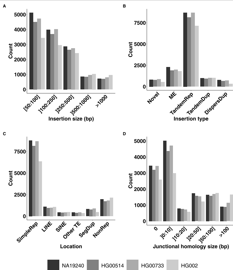
Fig. 2 Distributions of insertion variant features across several callsets. Distributions of a insertion size, b insertion type, c repeated context of insertion and d homology size at the breakpoint for NA19240, HG00514, HG00733 and HG002 insertion variant callsets. Abbreviations: SimpleRep for simple repeat, ME for mobile element, TandemRep for tandem repeat, TandemDup for tandem duplication, DispersDup for dispersed duplication
