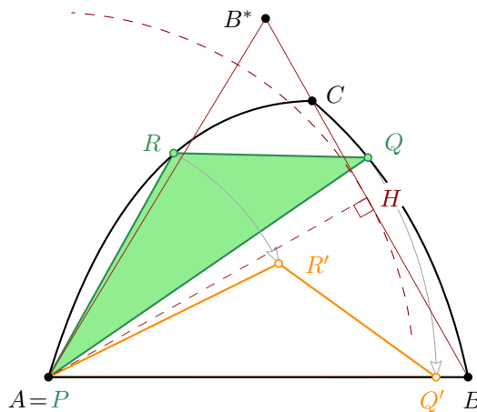
Figure 10: Proof of Theorem 6: |AR| \leq |AH| .
