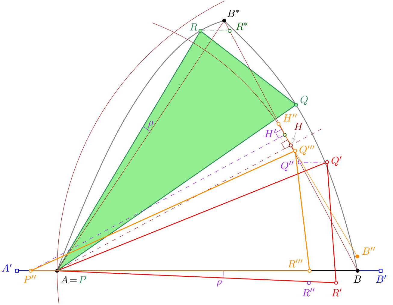
Figure 11: Proof of Theorem 6: the final case.
