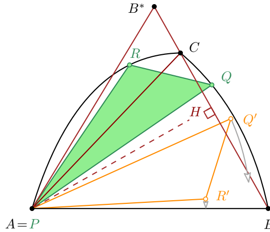
Figure 9: Proof of Theorem 6: R \in \triangle AHB^* .
