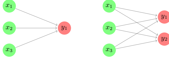
Fig. 1. Standard (left) and multiple (right) logistic regressions.
