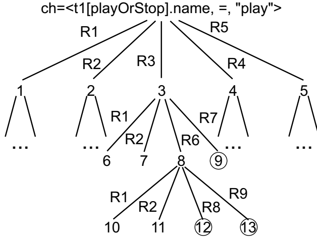
Fig. 6: Model state tree for a developer change.
