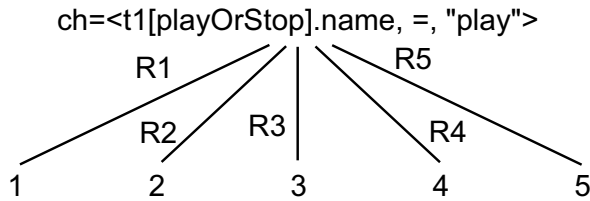
Fig. 5: Initial model state tree for a developer change
