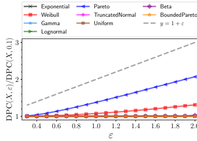
Figure 6: Expected cost of DYN-PROG-COUNT( X, \varepsilon ) as a function of \varepsilon for different distributions for X ( C = R = 360 s).
