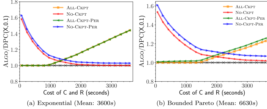
Figure 5: Expected costs of the different strategies normalized to that of DYN-PROG-COUNT( X, 0.1 ) when C = R vary, for Exponential and Bounded Pareto distributions.
