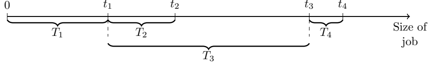
Figure 4: Illustration of job progress (and showing t_k versus T_k ) for the reservation sequence \mathcal{S} = \{(W_1, 1), (W_2, 0), (W_3, 1), (W_4, 0)\} .
