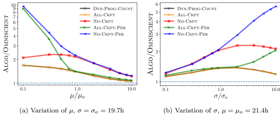
Figure 7: Normalized performance of algorithms with omniscient scheduler when \mu or \sigma vary. Basis is the LogNormal distribution in Fig. 1 ( \mu_o = 21.4\text{h} , \sigma_o = 19.7\text{h} ). C = R = 600\text{s} , \varepsilon = 1 . Black (DYN-PROG-COUNT) and yellow (ALL-CKPT) lines overlap.
