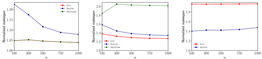
Figure 3: Performance for roofline model (left), communication model (middle) and Amdahl's model (right) with P = 7500 , \lambda = 10^{-7} and n \in [100, 1000] .
