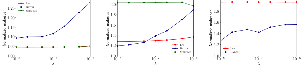
Figure 4: Performance for roofline model (left), communication model (middle) and Amdahl's model (right) with P=7500 , n=500 and \lambda \in [10^{-8}, 10^{-6}] .
