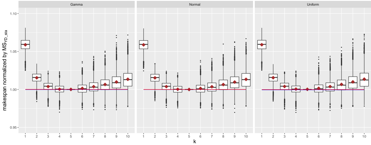
Figure 1: Performance (with boxplots) of the static strategy that chooses the value of k . Brown-red diamonds plot \mathbb{E}[MS_D](k) (theoretical makespan). The blue (resp. red) line represents the makespan obtained by the optimal dynamic strategy \overline{MS}_{sim\_dyn}(W_{th}) (resp. the YD-dynamic strategy \overline{MS}_{YD\_dyn} ).
