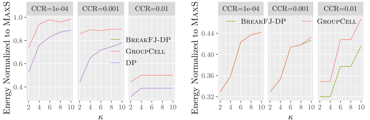
(a) Linear chains (BREAKFJ-DP and DP give the same results, hence only DP is visible).
