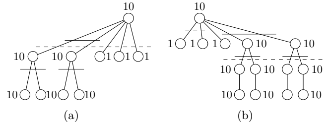
Figure 3: Two cases where SplitSubtrees is suboptimal. Dashed edges represent the solution of SplitSubtrees, plain edges give the optimal partition.
