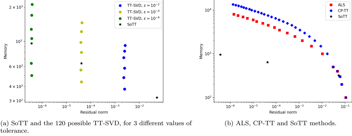
FIG. 8. Friedman function case, presented in Section 5.2.3, memory as function of the residual norm, in logarithmic scale for: a) and b).
