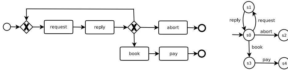
Figure 10: Process Model (V0): BPMN Process (left) and LTS Model (right).
