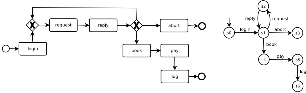
Figure 12: Process Model (V2): BPMN Process (left) and LTS Model (right).
