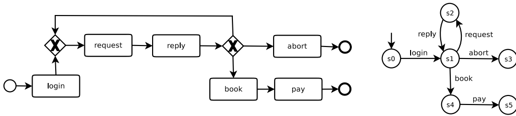
Figure 11: Process Model (V1): BPMN Process (left) and LTS Model (right).
