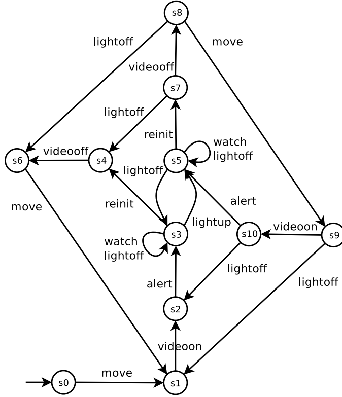
Figure 8: Case Study: Composition LTS.
