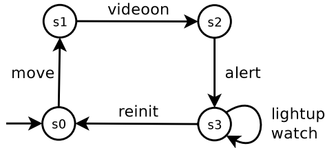
Figure 9: Case Study: Composition LTS (V2).
