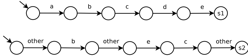
Figure 2: Example for the Path Similarity Criterion.
