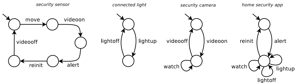
Figure 7: Case Study: Objects.
