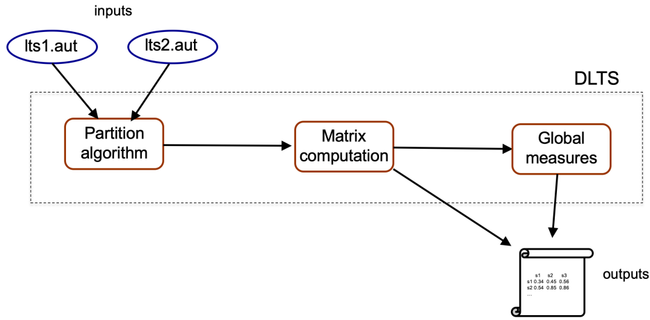
Figure 5: Tool Support.
