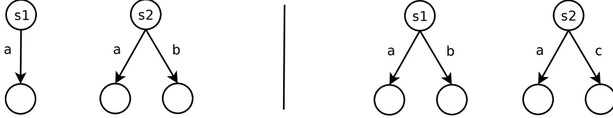
Figure 3: Example for the Transition Matching Criterion.
