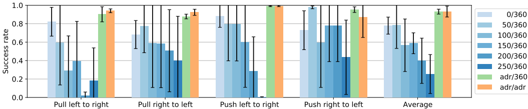
Figure 9: Success rate for multi-video policies trained with different randomization strategies using state trajectories from method A, and evaluated on the easy benchmark. Legend: the first number represents variability in the 3D position of the gripper, \sigma in mm; the second corresponds to the range of hand orientation in degrees. Five policies are trained for each parameter and we report mean and standard deviation (error bar in the plot).
