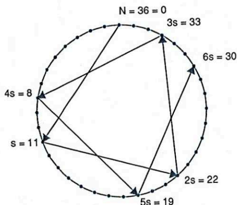
FIG. 1. An optimal loop network G(36; 1, 11) , d(36; 1, 11) = 9 = d(36) .
