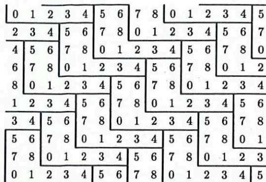
FIG. 2. Geometrical representation of G(9; 1, 7) .
