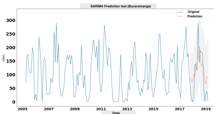
Figure 5: Time series prediction with real data from some sensors in Bucaramanga-Colombia
