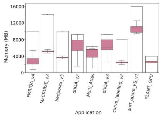
Fig. 1: Memory requests during submission and memory usage variation for nine representative medical and neuroscience applications.
