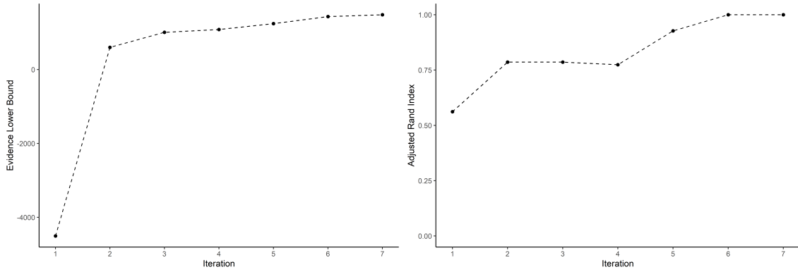
Figure 4: Left: Values of the evidence lower bound (ELBO) for successive iterations of the VEM algorithm during MAGMACLUST training. Right: The corresponding ARI values between predicted and true clusters for the same iterations. In this illustrative example, the algorithm reached convergence after 7 iterations only.
