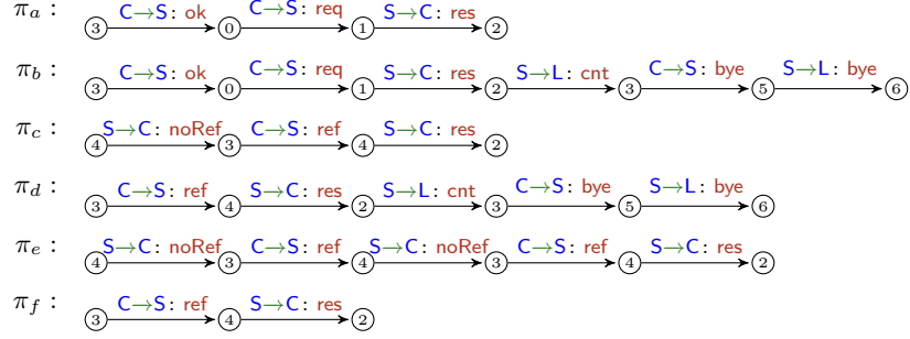
Fig. 1. Runs of \mathbb{C}ref .
