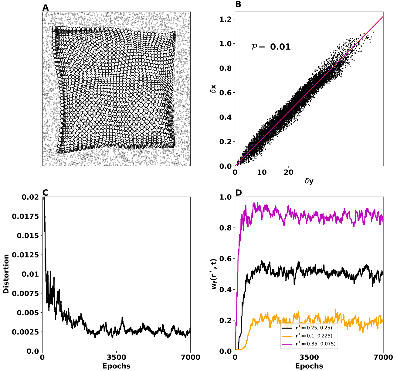
Figure 2: Two-dimensional SOM performance in the stable case. A Feed-forward weights (white discs) as they have been organized into a topographic map after 7000 epochs. The input in this case is a two-dimensional rectangular uniform distribution (black dots). B \delta x - \delta y representation (black cloud), mean of \delta x (red line), and the linear regression of the \delta x - \delta y representation (magenta line). The fact that the cloud is aligned around the red line indicates that the topographic map is well-organized, as confirmed by a good index performance \mathcal{P} = 0.01 . C Distortion indicates that the loss of information during the learning process decreases and the mapping of the input data to a two-dimensional self-organizing map respects the structure of the neighborhoods. D Temporal evolution of norm-2 of feed-forward weights of three neurons placed at r^* = (0.25, 0.25) , (0.1, 0.225) , and (0.35, 0.075) . Condition (15) is fulfilled and therefore the weights converge to an equilibrium giving rise to a well-formed topographic map.
