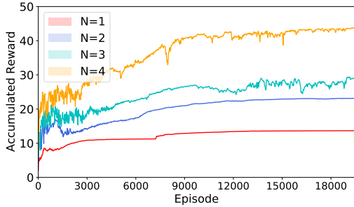
Fig. 7: Accumulated reward with training with \alpha = 1 .
