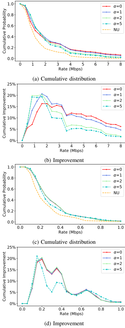
Fig. 9: Cumulative distribution and improvement on cumulative distribution of vehicles' access rate with N = 2 from 1:00 to 5:00 (a)-(b) and from 9:00 to 13:00 (c)-(d).
