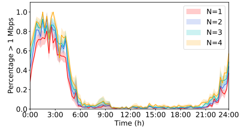
(a) Percentage of vehicles whose access rate is more than 1 Mbps
