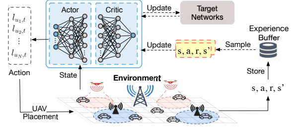
Fig. 3: DDPG for UAV dynamic placement.
