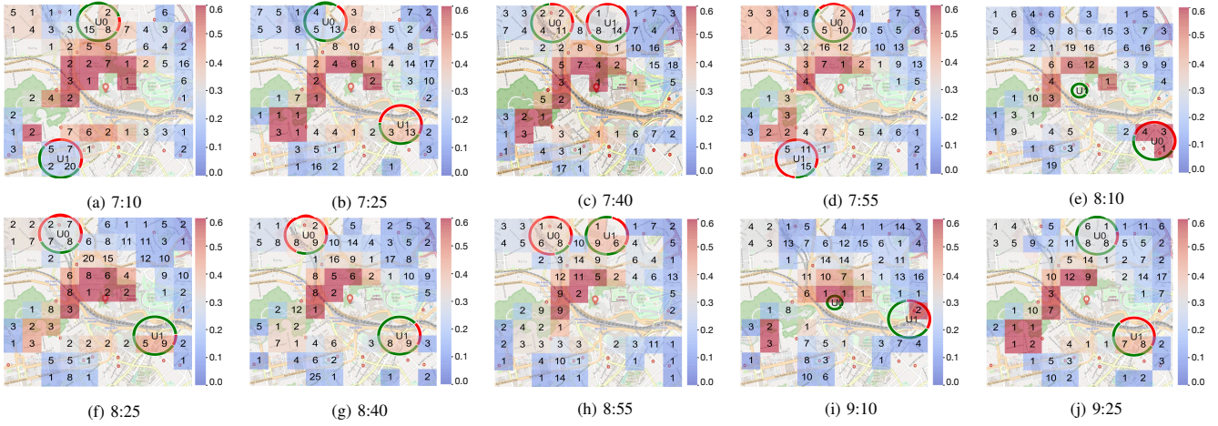
Fig. 6: Locations and battery left of UAVs with \alpha = 0 and N = 2 from 7:00 to 9:30.
