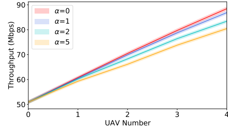
Fig. 10: Throughput with different numbers of UAVs and \alpha .
