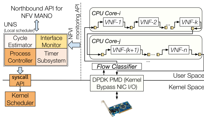
Fig. 2. System Architecture
