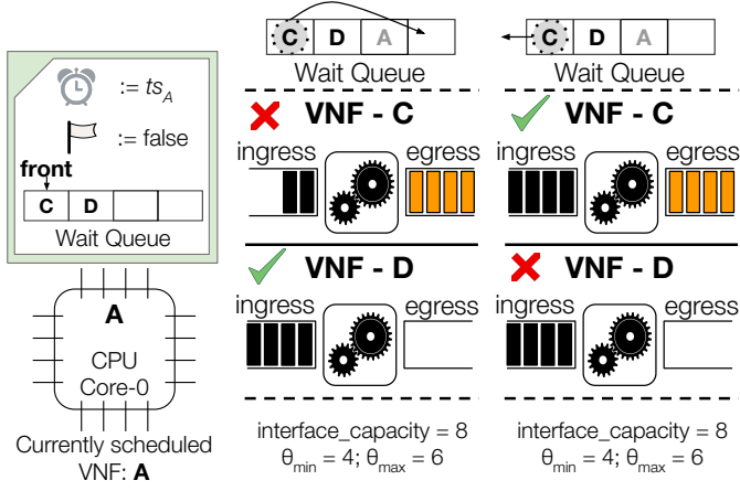
(a) State of data structures after initialization (b) VNF at the queue after front satisfies the selection criteria (c) VNF at the queue when front does not satisfy the selection criteria
