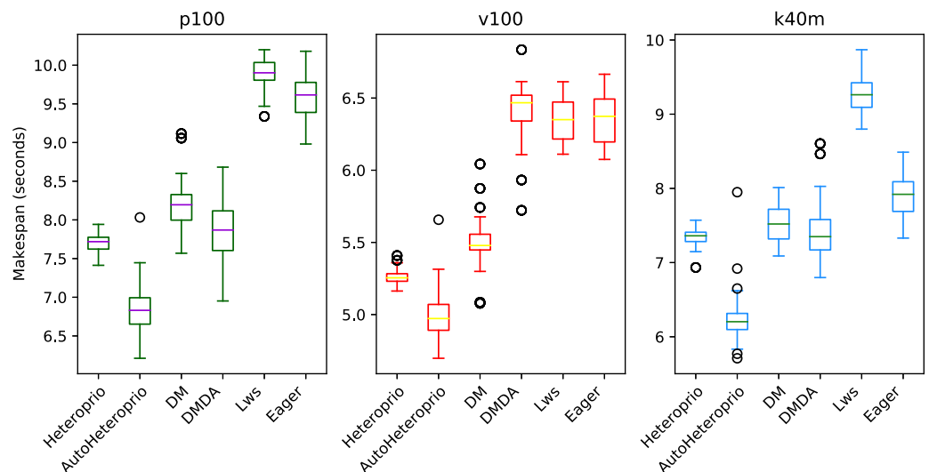
Figure 6 Execution times for QrMumps for different schedulers on the three configurations. The boxes show the distribution of the 32 makespans (896 for AutoHeteroprio) for each case.
