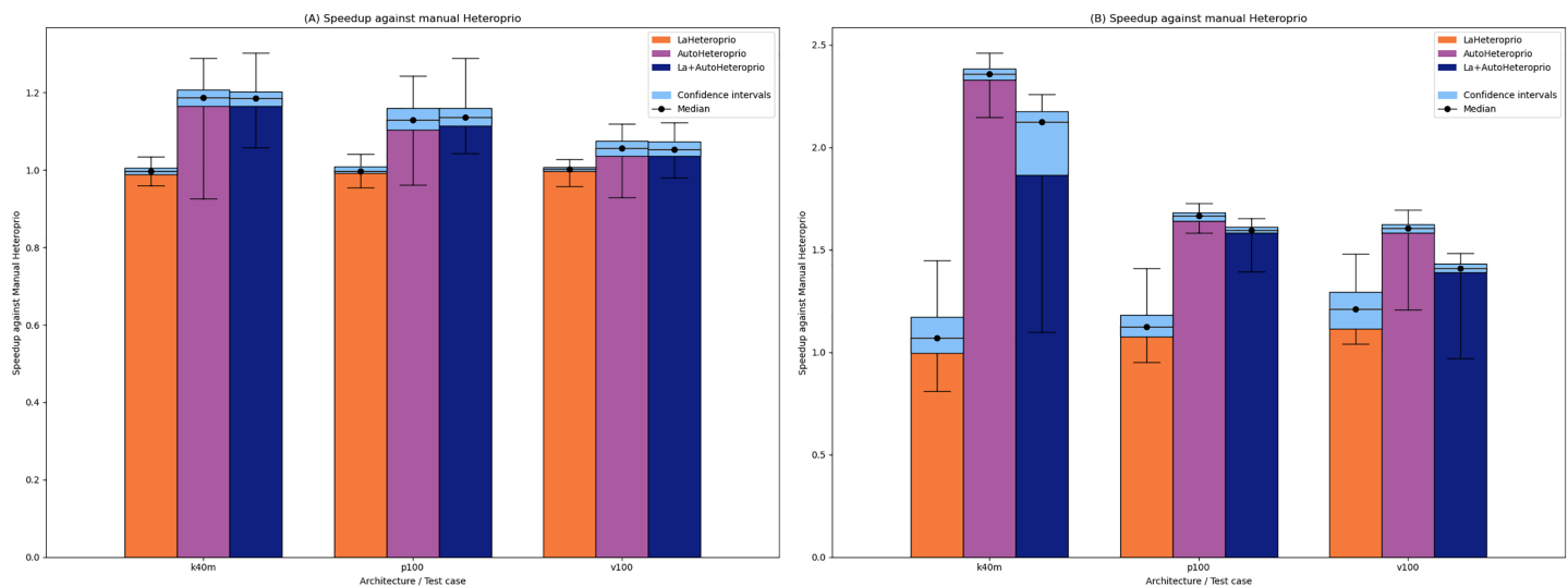
Figure 4 Speedups of LaHeterprio, AutoHeterprio, and LaAutoHeterprio against Heterprio in the Qr factorization (QrMumps) and the LU factorization (PaStiX). (A) Qr factorization (QrMUMPS). (B) LU factorization (PaStiX). The hatched area represents the interval of confidence of the 32 corresponding runs. Full-size DOI: 10.7717/peerj-cs.969/fig-4
