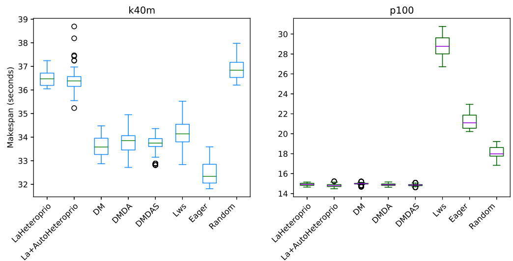
Figure 9 Execution times for Chameleon QR factorization for different schedulers on the p100 and the k40m configuration. The boxes show the distribution of the 32 makespans (896 for LaAutoHeterprio) for each scheduler.
