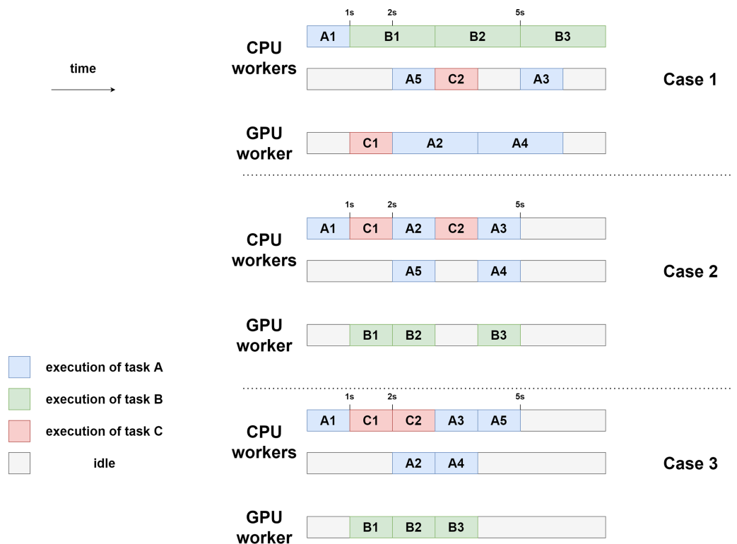
Figure 15 Example executions for the three different priority settings using two CPU workers and one GPU worker. Full-size DOI: 10.7717/peerj-cs.969/fig-15
