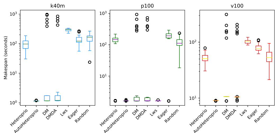
Figure 12 Execution times for the second ScalFMM test case on the three hardware configurations (k40m, p100 and v100). The scale of the Y-axis is logarithmic. The boxes show the distribution of the 32 makespans (896 for AutoHeteroprio) for each scheduler. Full-size DOI: 10.7717/peerj-cs.969/fig-12
