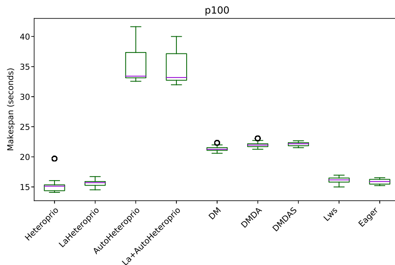
Figure 5 Execution times of the PaStiX solve step for different schedulers on the P100 configuration. The boxes show the distribution of the 32 makespans (896 for AutoHeteroprio and LaHeteroprio) for each scheduler. Full-size DOI: 10.7717/peerj-cs.969/fig-5
