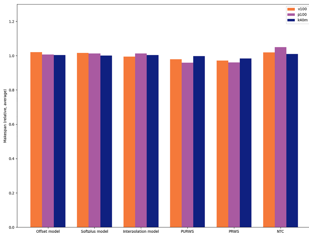
Figure 13 Relative difference between six heuristics in the case of the Cholesky factorization (Chameleon POTRF). Full-size DOI: 10.7717/peerj-cs.969/fig-13
