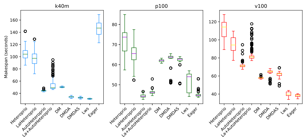
Figure 10 Execution times for PaStiX factorization for different schedulers on the three hardware configurations (k40m, p100 and v100). The boxes show the distribution of the 32 makespans (896 for AutoHeterprio and LaAutoHeterprio) for each scheduler.
