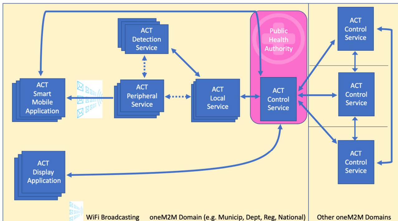
Figure 5.1-1: ACT Architecture
