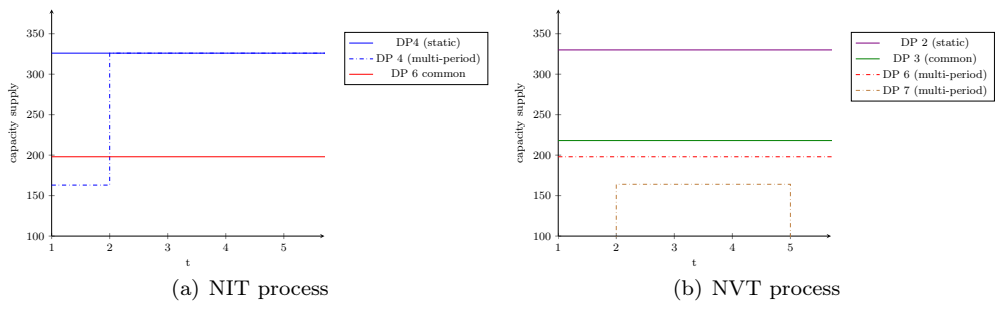
Figure 5: Capacity-allocation decisions from static modeling approach versus the a priori capacity C_t for 5-4/8/20-25-(I1,LT,TC,..)
