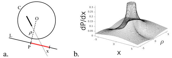
Fig. 5. PDF \frac{\partial P}{\partial x}(x) that a chord of circle C meets line L at coordinate x , with L at distance \rho from the centre of the circle.
