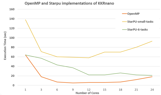
Fig. 3. Execution time for 693 iterations of TFQMR solver of KKRnano of original and StarPU-ized implementations.
