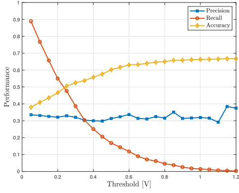
Fig. 5: Performance metrics of the threshold comparison method.
