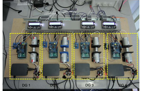
Fig. 2: The microgrid platform consisting of 4 DG units, where each DG unit is composed of one Raspberry Pi, one Arduino board, two motors and one light bulb to demonstrate the effect of voltage instability on the level of brightness [13].
