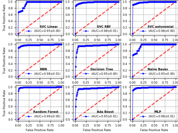
Fig. 7: ROC curves of the different machine learning algorithms.
