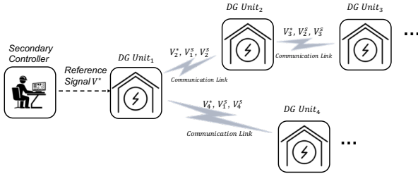
Fig. 1: A distributed and cooperative microgrid control system consisting of both primary and secondary controls. Interconnected DG Units can exchange data with neighboring DG units through sparse communication networks to transmit reference values and measurement values (denoted by the superscript s ) [10].
