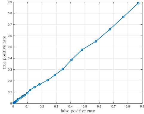
Fig. 6: ROC curve of a classifier based on threshold comparison applied to detect the MaR attack.
