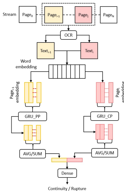
Figure 3: GRU Model architecture.
