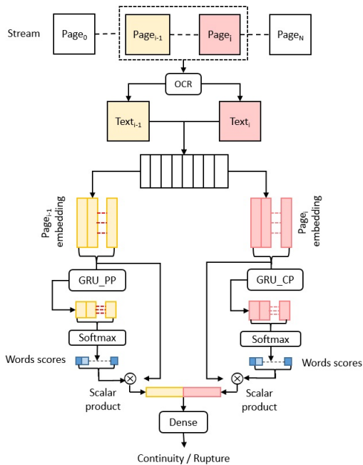
Figure 4: AGRU Model architecture
