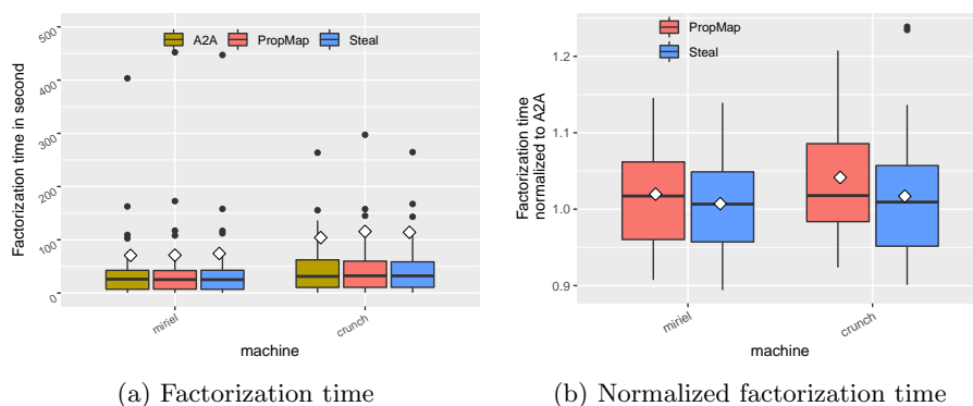
Figure 7: Factorization time ( left ), and that of PROPMAP and STEAL, normalized to ALL2ALL ( right ), on miriel and crunch . White diamonds represent mean values.
