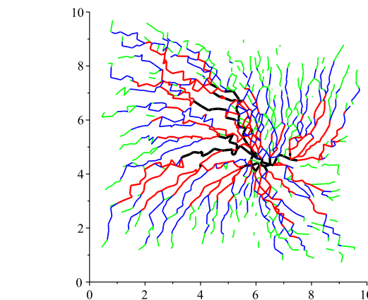
Figure 23: Map of segment densities in Delaunay Paris for the geo-routing path algorithm converging on a single destination point.
