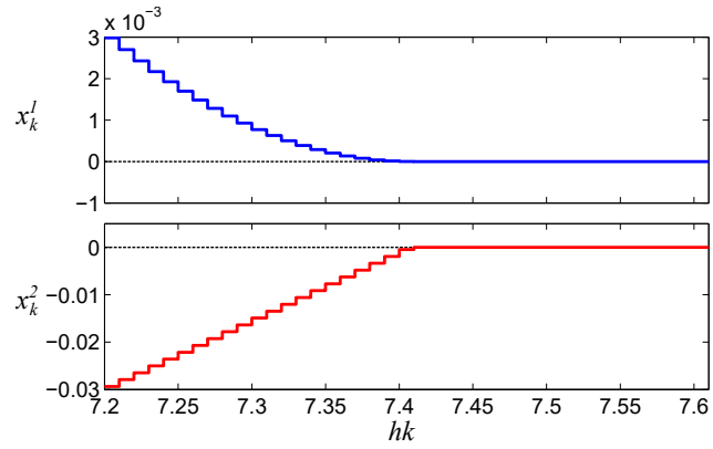
Figure 6: Close-up of the discrete-time approximation of (36).
