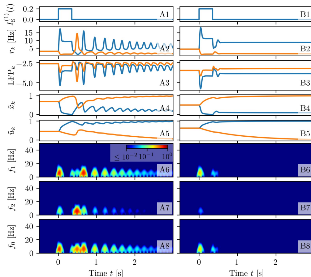
Fig 4. WM operations for a heuristic firing rate model. The results of two experiments are reported here for different background currents: WM maintenance via spontaneous reactivation of the target population ( I_B = 1.520 , A) and via a persistent asynchronous activity ( I_B = 2.05 , B). Profiles of the stimulation current I_s^{(k)}(t) for the excitatory populations (A1–B1). Population firing rates r_k(t) (A2–B2), local field potentials LFP_k defined in Eq (28) (A3–B3), normalized available resources \tilde{x}_k(t) (A4–C4) and normalized utilization factors \tilde{u}_k(t) (A5–C6) of the excitatory populations calculated from simulations of the firing rate model (19), (21). Spectrograms of the local field potentials: LFP_1(t) (A6–B6), LFP_2(t) (A7–B7), and LFP_0(t) (A8–B8). All the other parameter values as in Fig 3.
