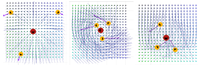
Figure 2: Examples of IF applied by the red agent during a simulation: each yellow agent is moved by the combination of their neighbours' IF (resulting vector in purple). Left) repulsion IF applied by every yellow agent in the pictures. Middle) circle-shape IF designed in Figure 1, middle. Right) the IF applied during simulation designed in Figure 1, right.
