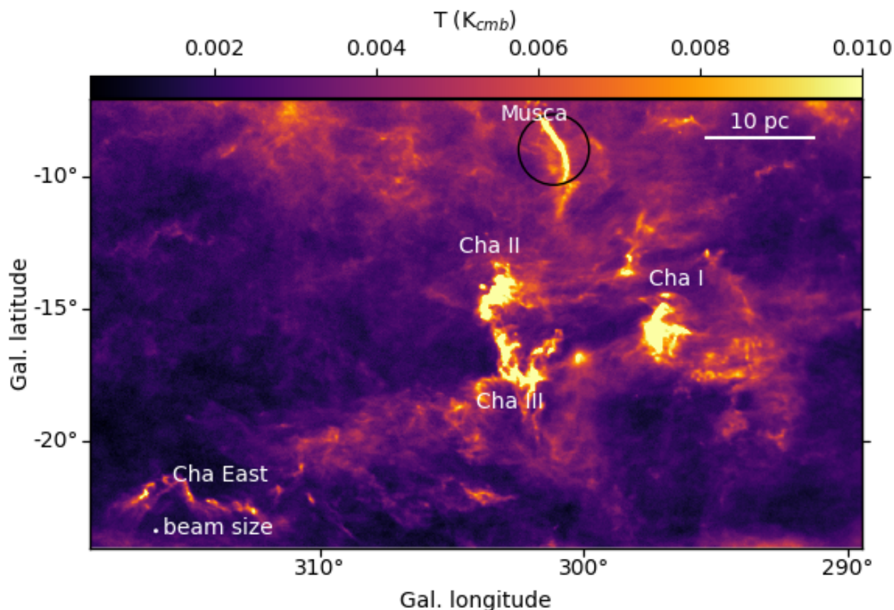
Fig. 1. Planck emission map at 353 GHz of the Chamealeon-Musca complex (Planck Collaboration et al. 2016a). The names of the relatively dense regions in the complex are indicated in white. The black circle indicates the region where GAIA data was extracted to investigate the distance of the Musca filament/cloud. The Planck resolution at 353 GHz is 4.8' , which corresponds to a physical size of 0.25 pc at a distance of 180 pc (Zucker et al. 2019).
