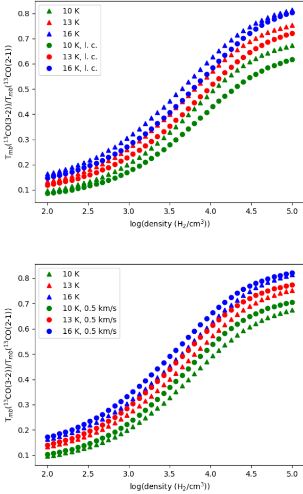
Fig. B.1. Top: Impact of a lower column density, namely N_{H_2} = 4 \cdot 10^{21} \text{ cm}^{-2} (indicated with l. c.) instead of N_{H_2} = 6 \cdot 10^{21} \text{ cm}^{-2} , on the ^{13}\text{CO}(3-2)/^{13}\text{CO}(2-1) ratio as a function of the density. Bottom: The impact of a lower FWHM ( 0.5 \text{ km s}^{-1} instead of 0.7 \text{ km s}^{-1} ) on the ^{13}\text{CO}(3-2)/^{13}\text{CO}(2-1) ratios as a function of the density. For both the width and the column density, their impact is plotted for 3 different temperatures: 10 K, 13 K and 16 K. This shows that the impact of these two variables is smaller than the uncertainty related to the temperature.
