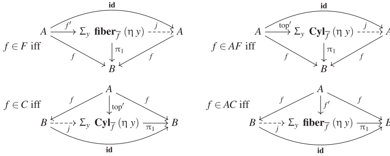
Figure 5. Diagrammatic illustration of Proposition 27.
