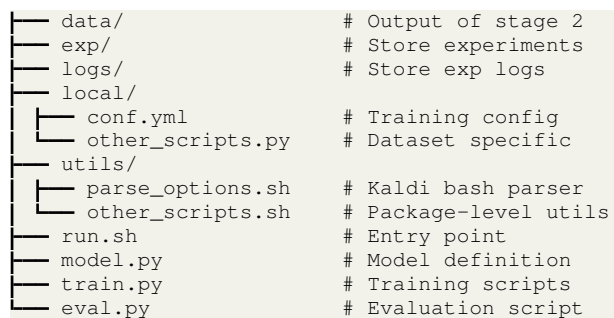
Figure 3: Typical directory structure of a recipe.
