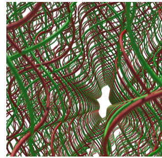
(f) The resulting net in \mathbb{R}^3 when the tile boundaries are taken as trajectories in Euclidean 3-space.
