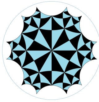
(b) The symmetries of the D -surface within a unit cell in \mathbb{H}^2 . Each line represents a mirror symmetry.
