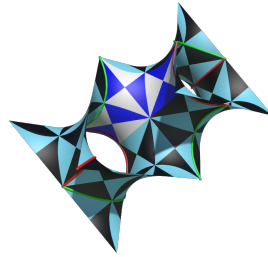
(e) The decoration from (d) and a fundamental domain shown as a decoration of the Diamond triply-periodic minimal surface. The triangles illustrate the symmetries of the surface.
