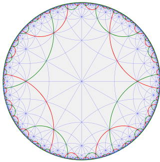
(d) A tiling of the hyperbolic plane with symmetry group 22222, represented by the green and red edges, with a tiling by triangles with \star 246 symmetry shown in blue in the background.
