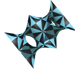
(c) A section of the D -surface in \mathbb{R}^3 , together with its smallest asymmetric triangle patches.
