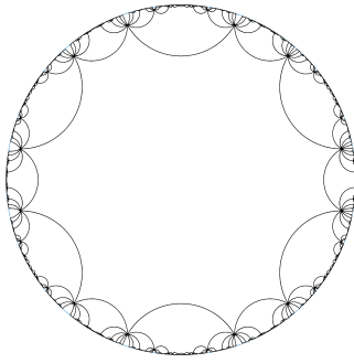
(a) Tessellation of \mathbb{H}^2 by dodecagons corresponding to the genus 3 Riemann surface that gives rise to the D -surface.
