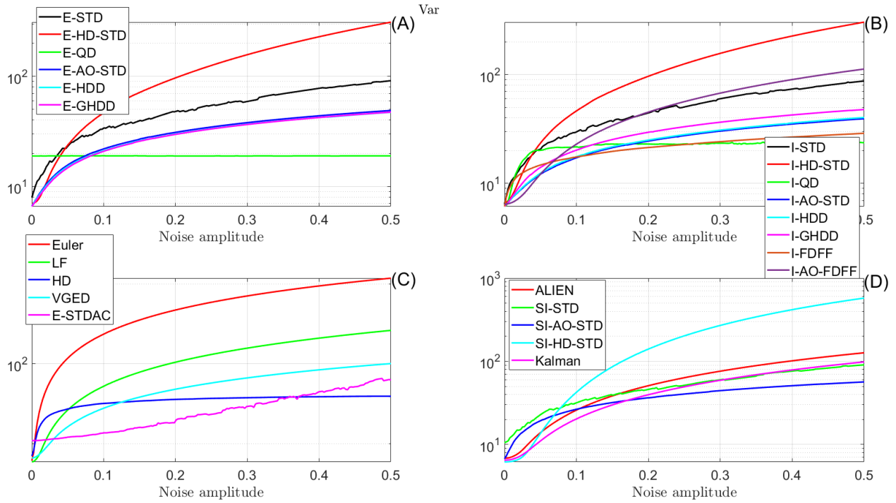
Figure 35: Variation for the first-order differentiation with respect to noise amplitude. Input noise: A \sin(20t) , A is the noise amplitude. Parameters are shown in Table 6 ( h = 50\text{ms} ).
