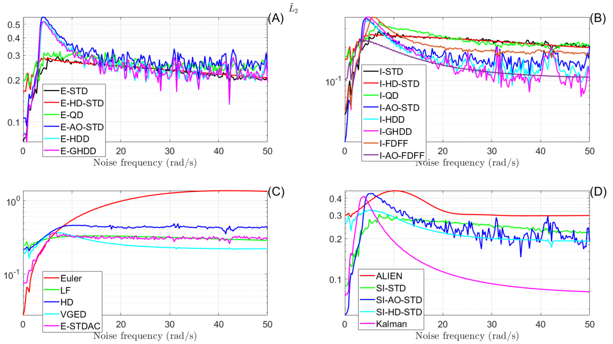
Figure 28: \tilde{L}_2 for the first-order differentiation with respect to noise frequency. Input noise: 0.05\sin(\omega t) , \omega is the noise frequency. Parameters are shown in Table 6 ( h = 50\text{ms} ).
