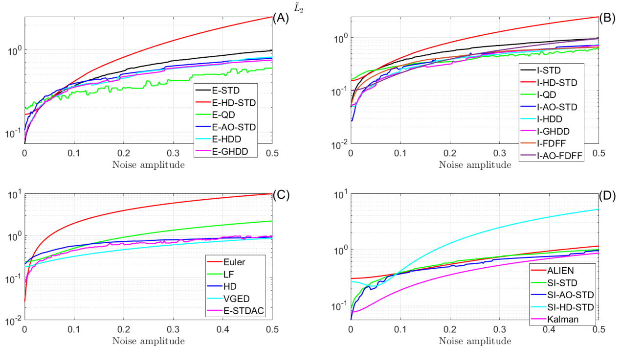
Figure 33: \tilde{L}_2 for the first-order differentiation with respect to noise amplitude. Input noise: A \sin(20t) , A is the noise amplitude. Parameters are shown in Table 6 ( h = 50\text{ms} ).
