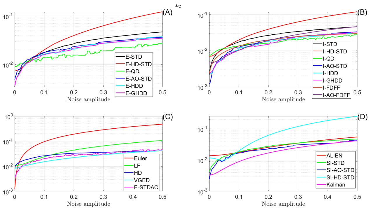
Figure 32: \bar{L}_2 for the first-order differentiation with respect to noise amplitude. Input noise: A \sin(20t) , A is the noise amplitude. Parameters are shown in Table 6 ( h = 50\text{ms} ).
