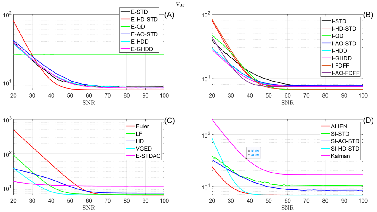
Figure 52: Variation for the first-order differentiation with respect to SNR of the white noise in the presence of initial error. Parameters are shown in Table 13 ( h = 50\text{ms} ).
