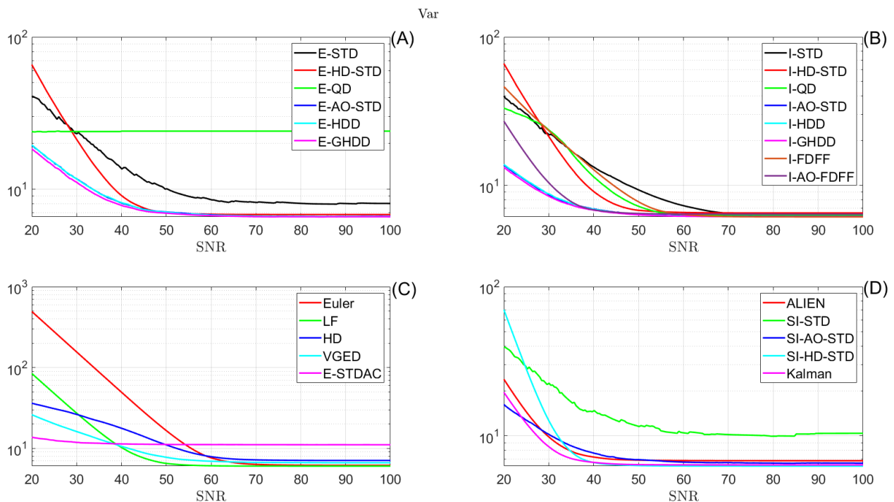
Figure 23: Variation for the first-order differentiation with respect to SNR of the white noise. Parameters are shown in Table 3 ( h = 50 ms).
