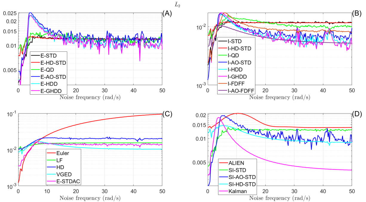
Figure 27: \bar{L}_2 for the first-order differentiation with respect to noise frequency. Input noise: 0.05\sin(\omega t) , \omega is the noise frequency. Parameters are shown in Table 6 ( h = 50\text{ms} ).
