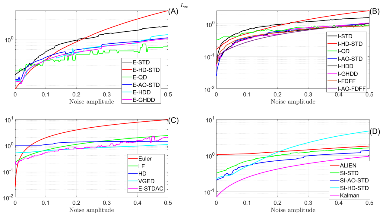
Figure 34: L_\infty for the first-order differentiation with respect to noise amplitude. Input noise: A \sin(20t) , A is the noise amplitude. Parameters are shown in Table 6 ( h = 50\text{ms} ).
