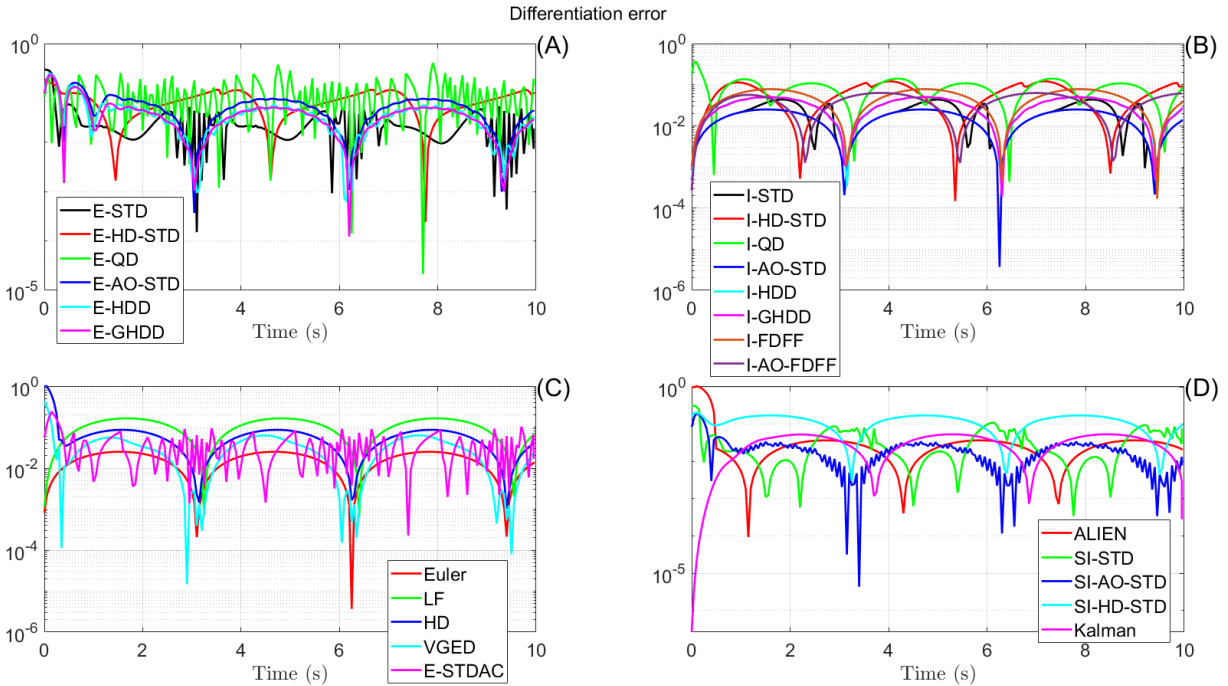
Figure 17: Error of the first-order differentiation under a noise-free condition. Parameters are shown in Table 3 ( h = 50\text{ms} ).
