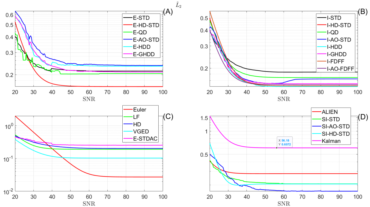
Figure 50: \tilde{L}_2 for the first-order differentiation with respect to SNR of the white noise in the presence of initial error. Parameters are shown in Table 13 ( h = 50\text{ms} ).
