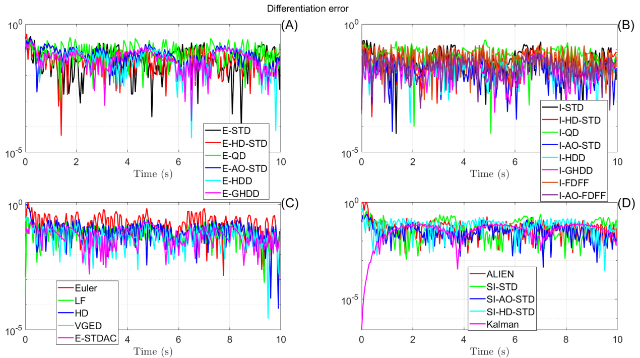
Figure 39: First-order differentiation error under a bell-shaped noise ( h = 50\text{ms} ).
