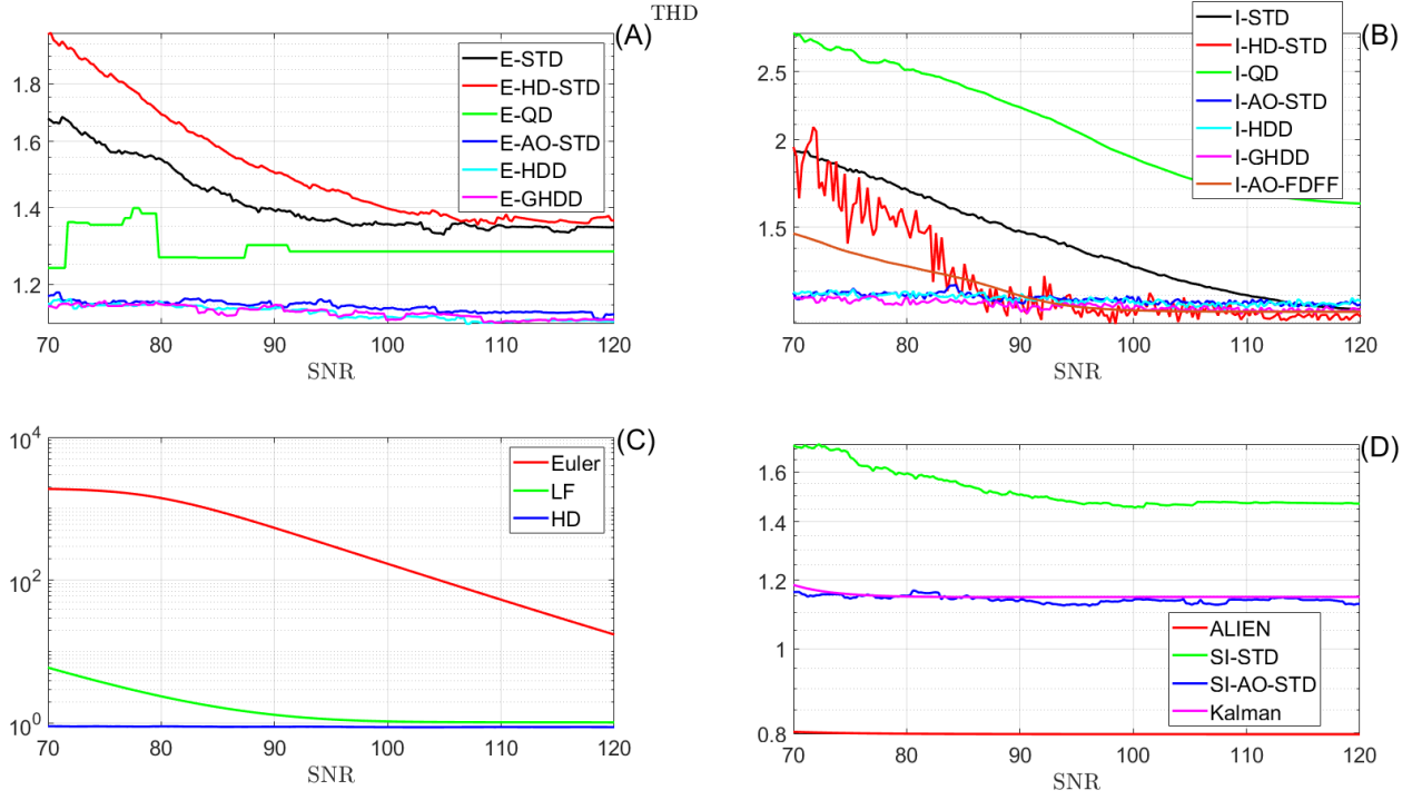
Figure 60: THD for the third-order differentiation under different SNRs ( h=10\text{ms} ).
