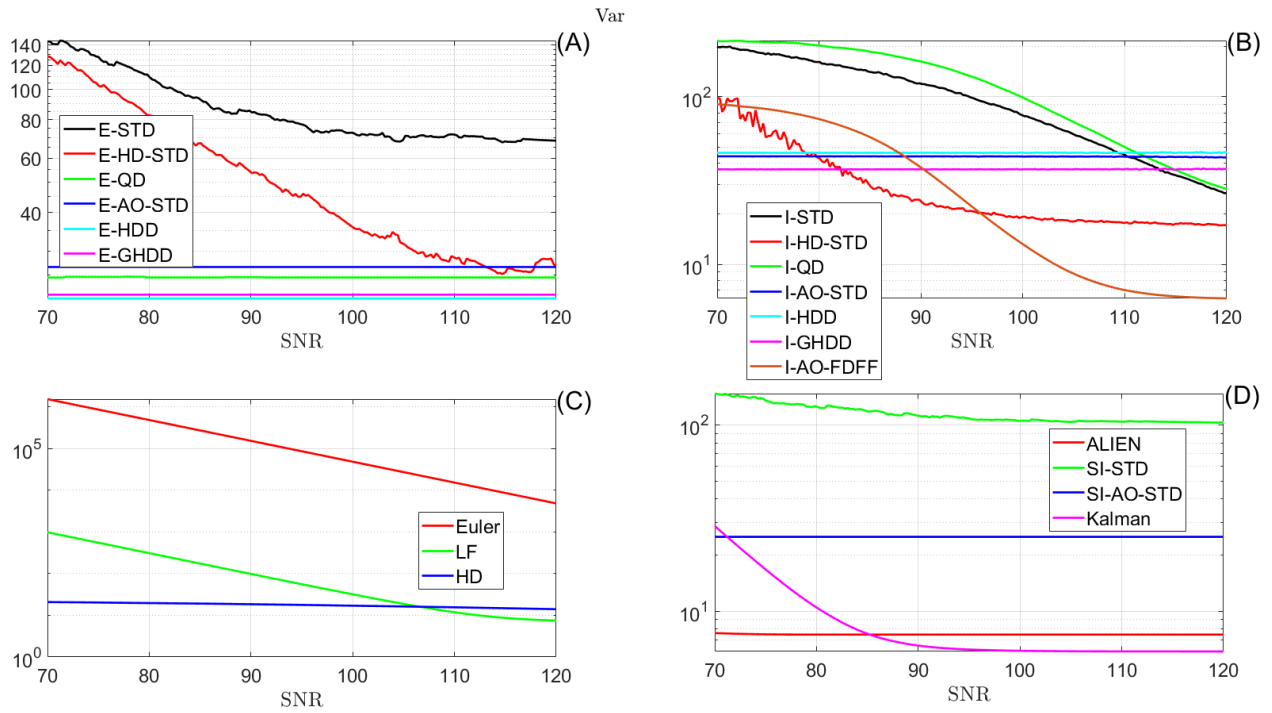
Figure 59: Variation for the third-order differentiation under different SNRs ( h = 10\text{ms} ).
