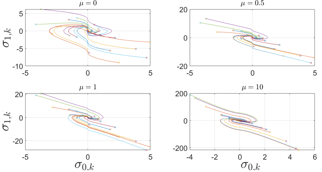
Figure 6: Phase-portrait of the I-HD-STD. Input signal is \sin(t) . \lambda_1 = 2, \lambda_2 = 2, h = 1\text{ms} .
