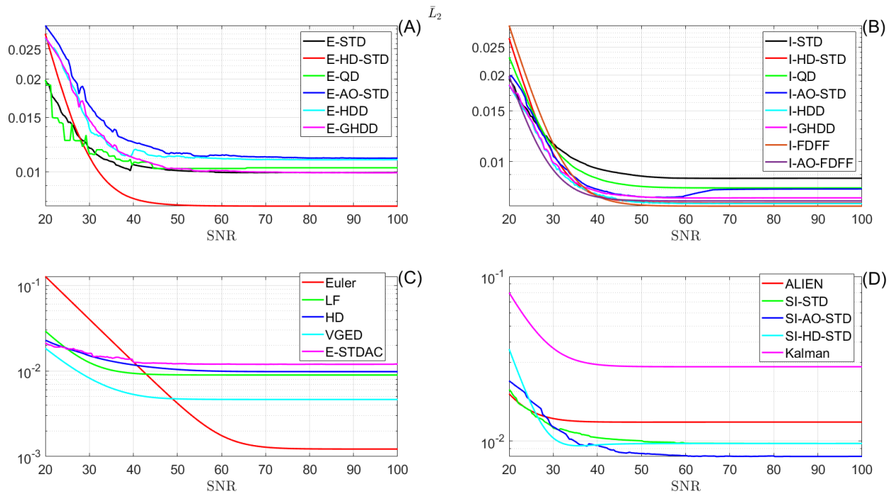
Figure 49: \bar{L}_2 for the first-order differentiation with respect to SNR of the white noise in the presence of initial error. Parameters are shown in Table 13 ( h = 50\text{ms} ).
