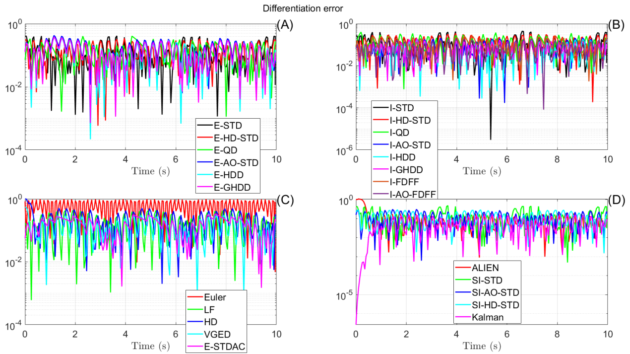
Figure 26: Error of the first-order differentiation under sinusoidal noise 0.05\sin(20t) . Parameters are shown in Table 6 ( h = 50\text{ms} ).
