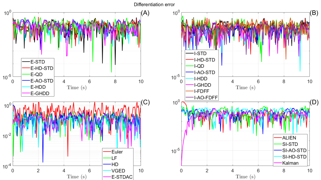
Figure 19: Error of the first-order differentiation in the presence of white noise. Parameters are shown in Table 3 ( h = 50\text{ms} , \text{SNR}=30\text{dB} ).
