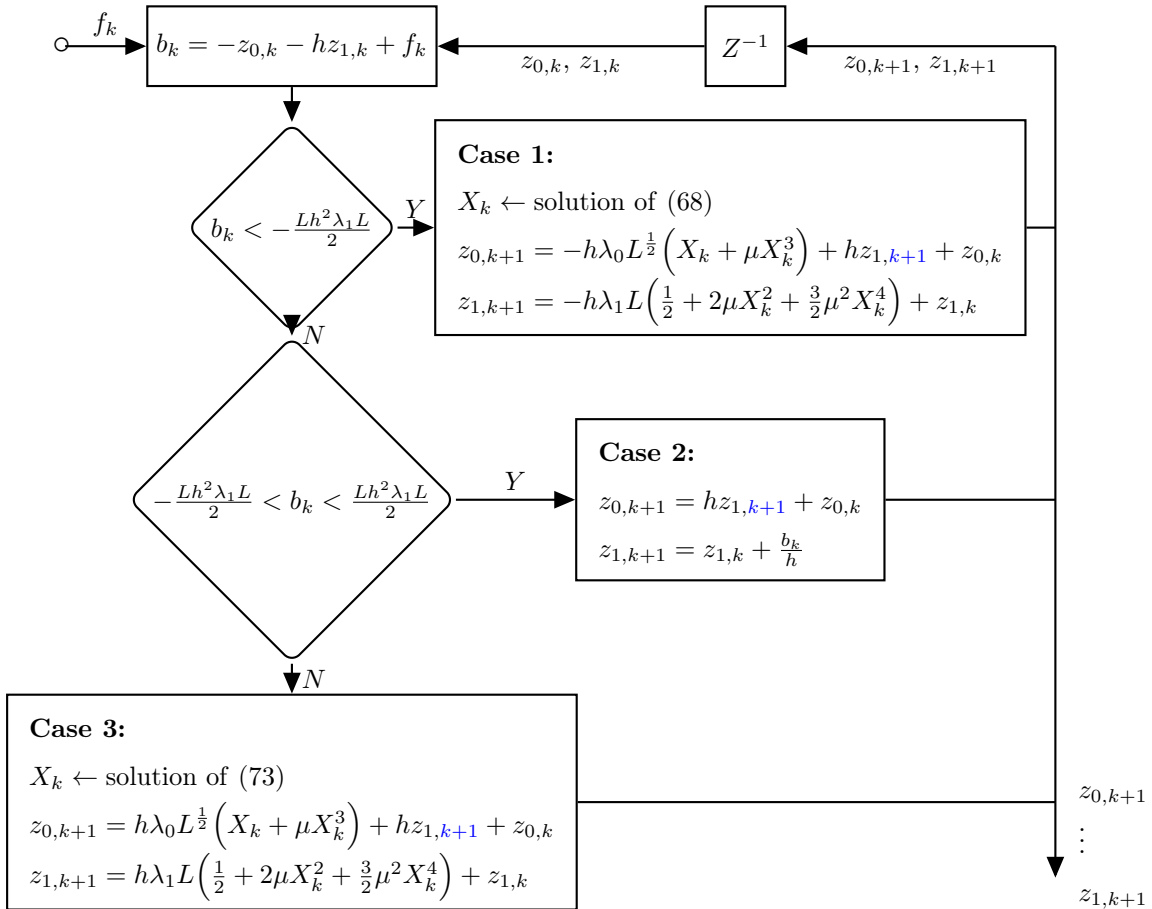
Figure 5: Flowchart of the I-HD-STD. The block Z^{-1} indicates one-step delay.
