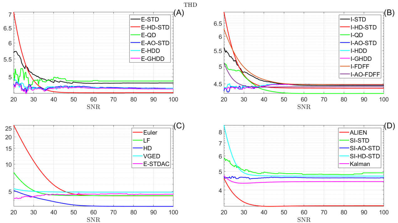
Figure 24: THD for the first-order differentiation concerning SNR. Parameters are shown in Table 3 ( h = 50\text{ms} ).
