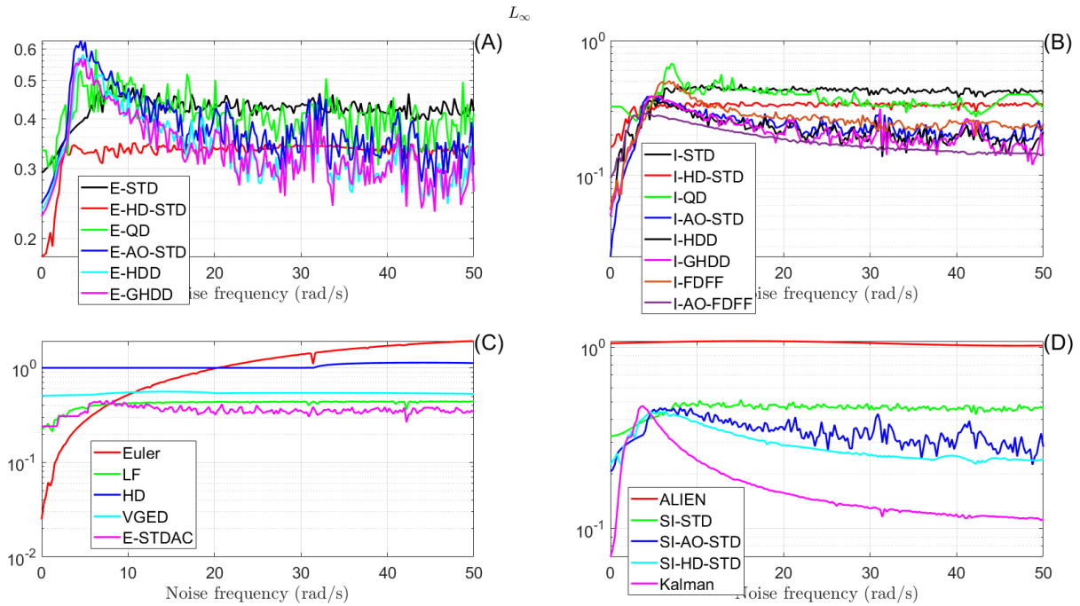
Figure 29: L_\infty for the first-order differentiation with respect to noise frequency. Input noise: 0.05\sin(\omega t) , \omega is the noise frequency. Parameters are shown in Table 6 ( h = 50\text{ms} ).
