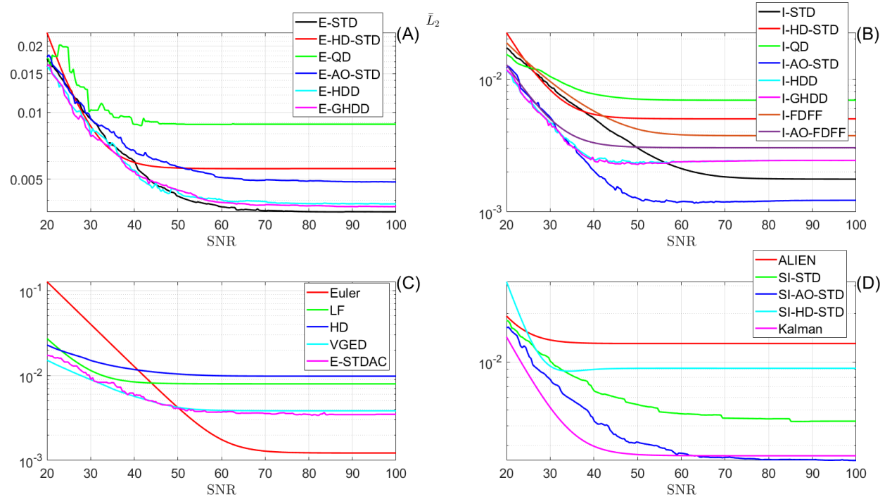
Figure 20: \bar{L}_2 for the first-order differentiation with respect to SNR of the white noise. Parameters are shown in Table 3 ( h = 50\text{ms} ).
