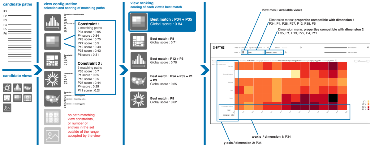
Fig. 5. Process for generating a default view.
