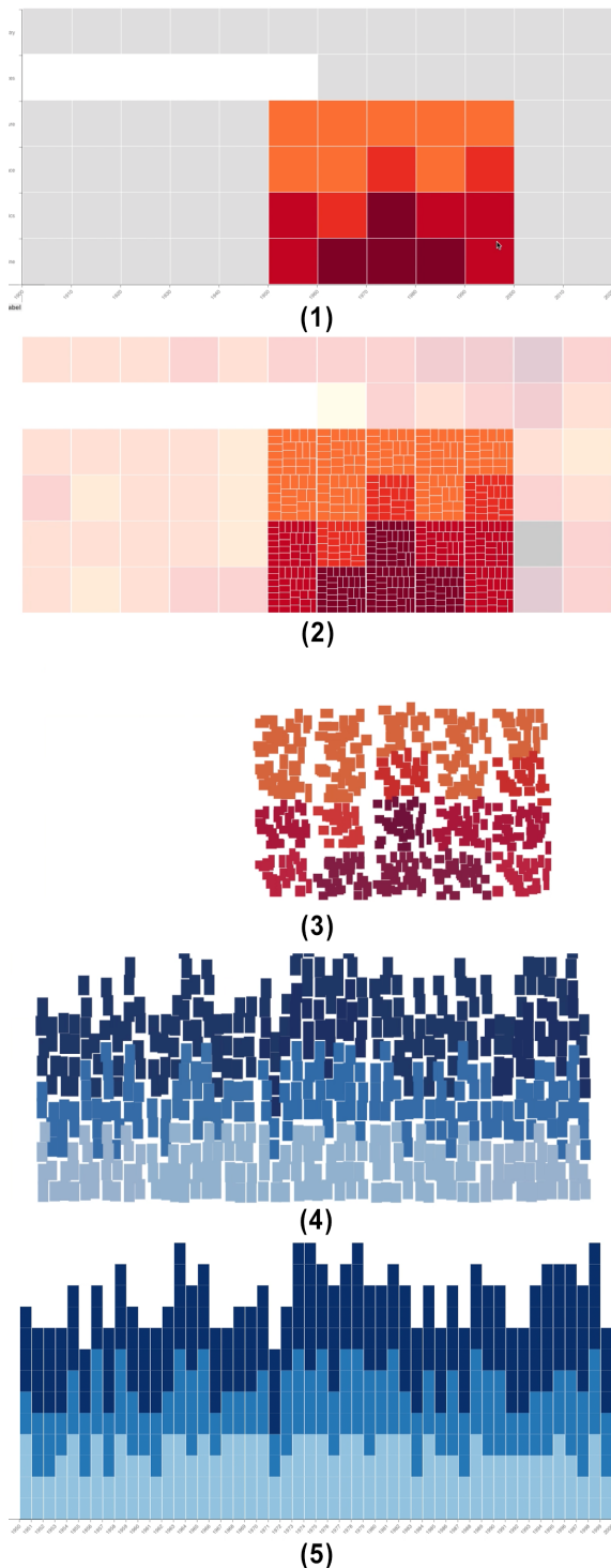
Fig. 7. Animated transition from a sub-selection made in a 2D density plot showing counts for types of Award File aggregated by decade (1), to a histogram showing the distribution of prizes per discipline for each individual year (5). Sample intermediate frames: (2) elements no longer present in the target view are faded out, and visual marks corresponding to aggregates get decomposed into groups that will transition towards the same target; (3-4) elements present in both the source and target views get smoothly interpolated along relevant encoding channels: position, color, shape; (5) elements that did not exist in the source view fade in.
