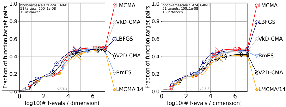
Figure B.2: Bootstrapped runtime distributions of a variety of large-scale solvers, taken from [25]. Shown are 51 targets in 10^{[-8..2]} for all functions of the bbob-largescale suite in dimension 160 (left) and 640 (right).
