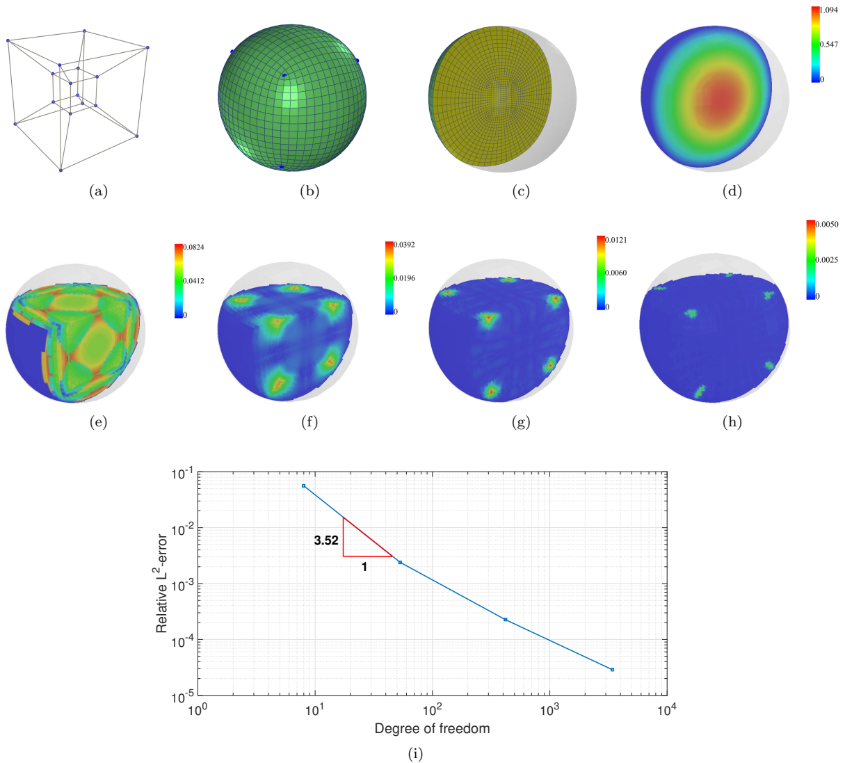
Figure 7: Convergence study on a sphere-like domain. (a): input control mesh; (b): interpolatory Catmull-Clark subdivision volume with the PIA method; (c): the interior view of (b); (d): reference solution to heat conduction problems; (e): error colormap of numerical solution on the level-0 subdivision volume; (f): error colormap of numerical solution on the level-1 subdivision volume; (g): error colormap of numerical solution on the level-2 subdivision volume; (h): error colormap of numerical solution on the level-3 subdivision volume; (i): convergence rate of relative L_2 error vs the number of degrees of freedom.
