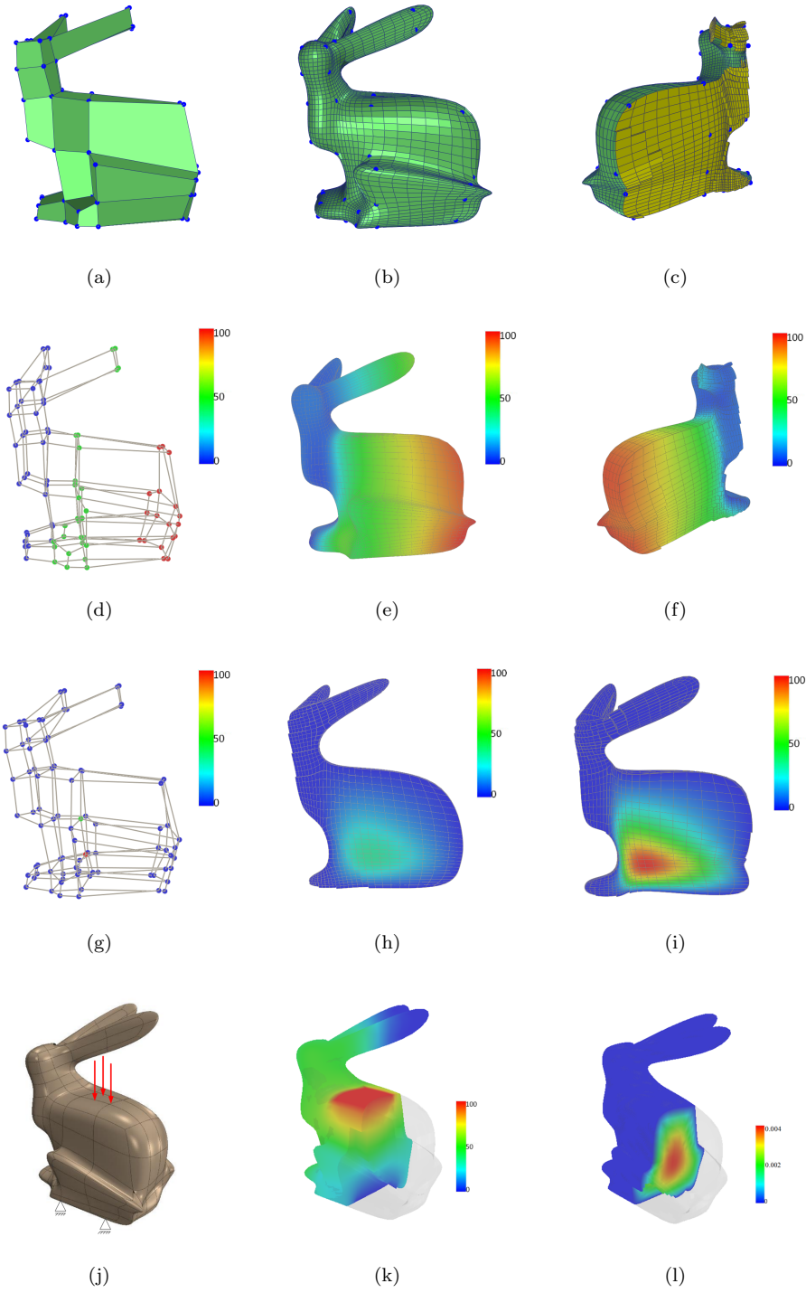
Figure 8: Bunny model. (a): The original mesh; (b): interpolatory volumetric subdivision result with the PIA method; (c): the interior view of (b); (d): the original control lattice with different material values, where blue, green and red correspond to 0, 50 and 100, respectively; (e) and (f): material distribution of the interpolatory subdivision solids by the PIA method; (g) the original control lattice with another set of material values at vertices; (h) material distribution of approximation Catmull-Clark subdivision volume with input (g); (i) material distribution of interpolatory Catmull-Clark subdivision volume with input (g); (j): boundary condition for linear elasticity simulation; (k): IGA results for linear elasticity simulation with boundary condition (j); (l): IGA results for heat conduction simulation.
