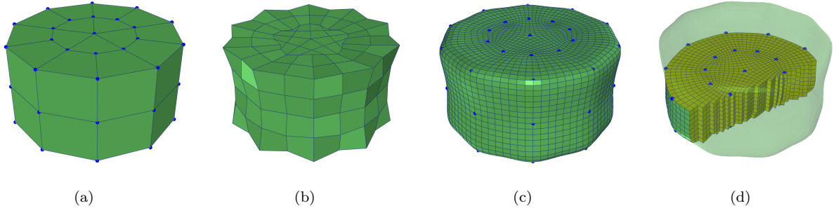
Figure 1: Interpolatory Catmull-Clark volumetric subdivision example with the push-back method. (a) The original mesh; (b) new control lattices constructed by the push-back operation; (c) subdivision result after two levels of Catmull-Clark volumetric subdivision from the modified control lattice; (d) the interior view of the result.
