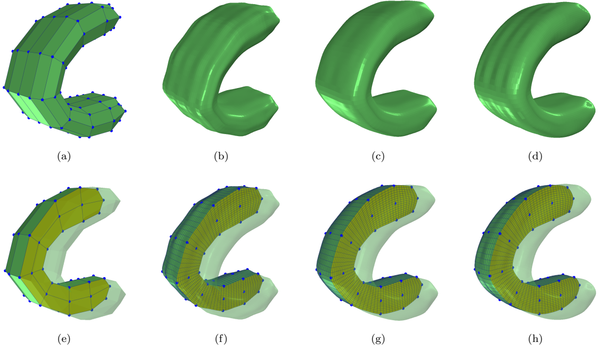
Figure 2: Examples of the push-back method with different parameters. (a) and (e): The original mesh; (b) and (f): interpolatory subdivision volume with \lambda_{ij} = 0.05 , \mu_F = 0.05 and \gamma_C = 0.05 ; (c) and (g): interpolatory subdivision volume with \lambda_{ij} = 0.25 , \mu_F = 0.125 and \gamma_C = 0.0625 ; (d) and (h): interpolatory subdivision volume with \lambda_{ij} = 0.25 , \mu_F = 0.25 and \gamma_C = 0.25 .
