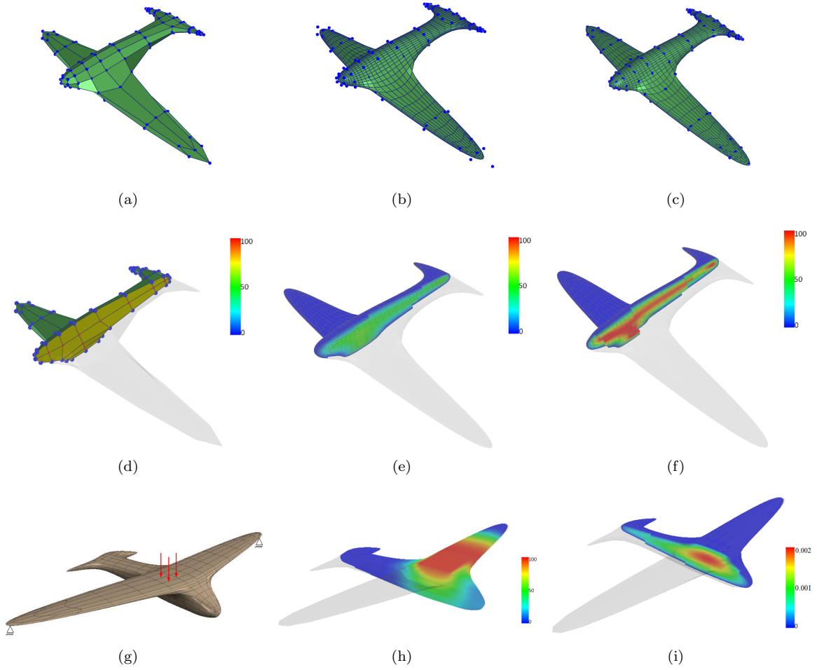
Figure 9: Airplane model. (a): Input control lattice; (b): Catmull-Clark subdivision volume after three subdivision steps; (c): interpolatory Catmull-Clark subdivision volume after three subdivision steps with the PIA method; (d): the original control lattice with different material values at vertices, where blue vertices have material value 0 and red vertices have material value 100; (e): material distribution of approximation Catmull-Clark subdivision volume after three subdivision steps; (f): material distribution of interpolatory Catmull-Clark subdivision volume after three subdivision steps; (g): boundary condition for linear elasticity simulation; (h): IGA results for linear elasticity simulation with boundary condition (g); (i): IGA results for heat conduction simulation.
