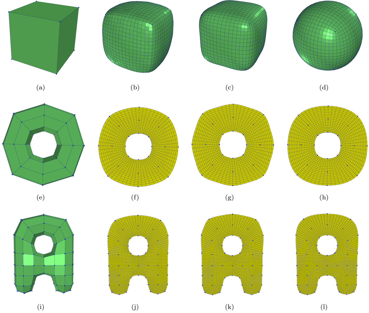
Figure 4: Comparison examples. From left to right: The input hexahedral mesh; the butterfly interpolatory subdivision method; the push-back method; and the PIA method.
