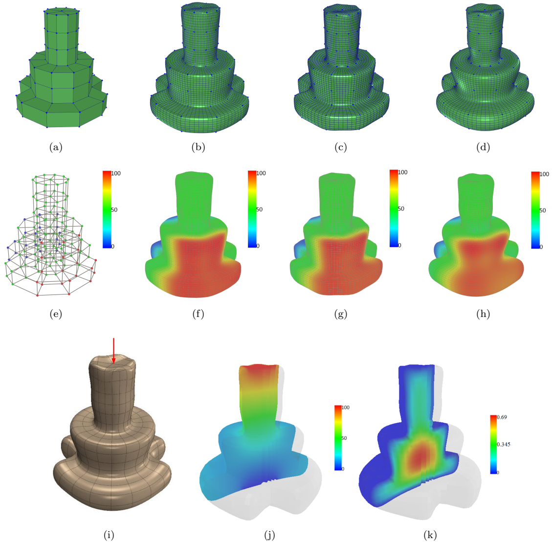
Figure 5: Comparison examples. (a-h): The input hexahedral mesh; the butterfly interpolatory subdivision method; the push-back method; and the PIA method. Blue, green and red vertices in (e) are assigned with material value 0, 50 and 100 respectively. (f-h): The corresponding material description over (b), (c) and (d) geometry, respectively. (i): Boundary condition for linear elasticity simulation on the interpolatory subdivision volume with the PIA method in (d); (j): IGA results for linear elasticity simulation with boundary condition in (i); (k): IGA results for heat conduction simulation.
