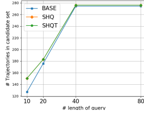
■ Figure 4 The average number of trajectories in candidate set in each method vs length of query in Facebook dataset. For both SHQ and SHQT the candidate set \tilde{\Gamma} is the same.
