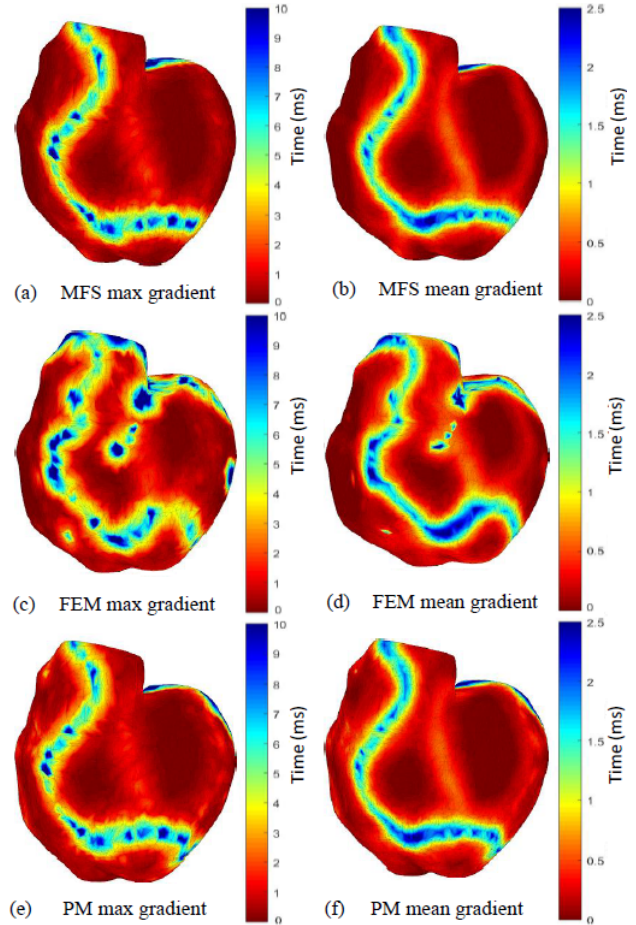
Figure 3: Reconstructed (MFS, FEM and PM) gradient maps calculated with the max and mean methods in the case of no tissue damage.
