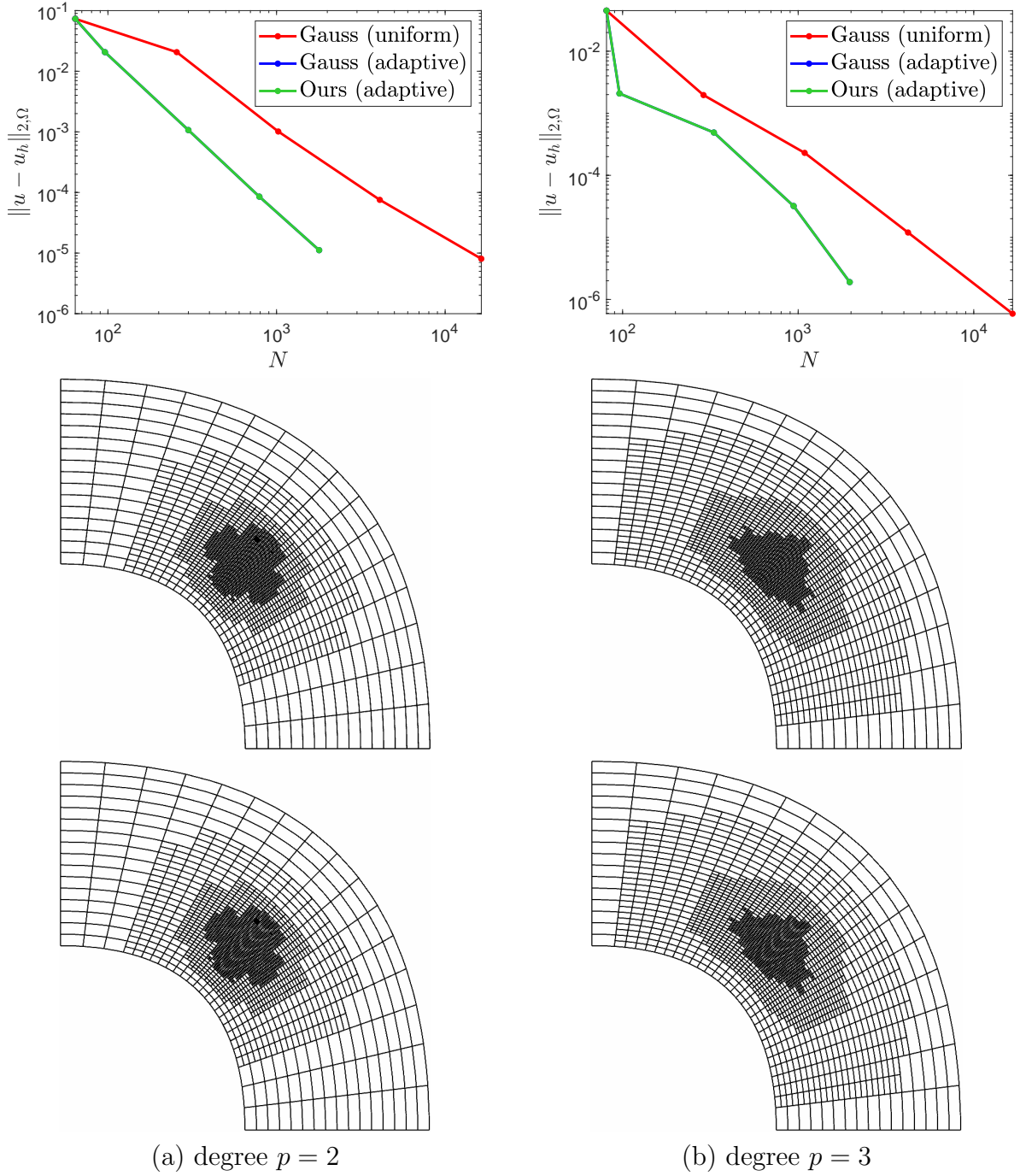
Figure 10: Convergence of error in L^2 norm with respect to degree p = 2 (left) and p = 3 (right) for the quarter annulus-shaped domain. The first row shows the error plots for uniform refinement by Gauss quadrature, adaptive refinements by Gauss quadrature and our method. Note that the latter two curves are visually indistinguishable. The second and last row present the hierarchical meshes on the computational domain obtained via adaptive refinement by Gauss quadrature and our method, respectively.
