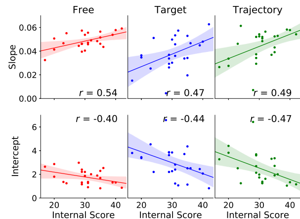
Fig. 11. Scatter plots with linear regression lines between the internal score of the IPC test and the regression coefficient terms obtained between the FoC ratings and Weight for each participant (slope (top) and intercept (down)). Translucent bands indicate 95% CIs. 10,000 bootstrap samples were used to estimate each 95% CI.
