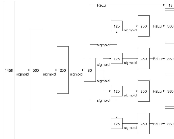
Fig. 4: Structure of the auto-encoder
