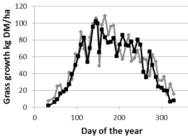
Left Clonakility 2015, RMSE 13.8 kg DM/ha, CCC 0.89 Right Ballyhaise 2013, RMSE 12.0 kg DM/ha, CCC 0.90 Figure 1: Comparison between the growths recorded in PBI (grey) and predicted by the MoSt model (black) for two contracting years in two contrasting farms.
